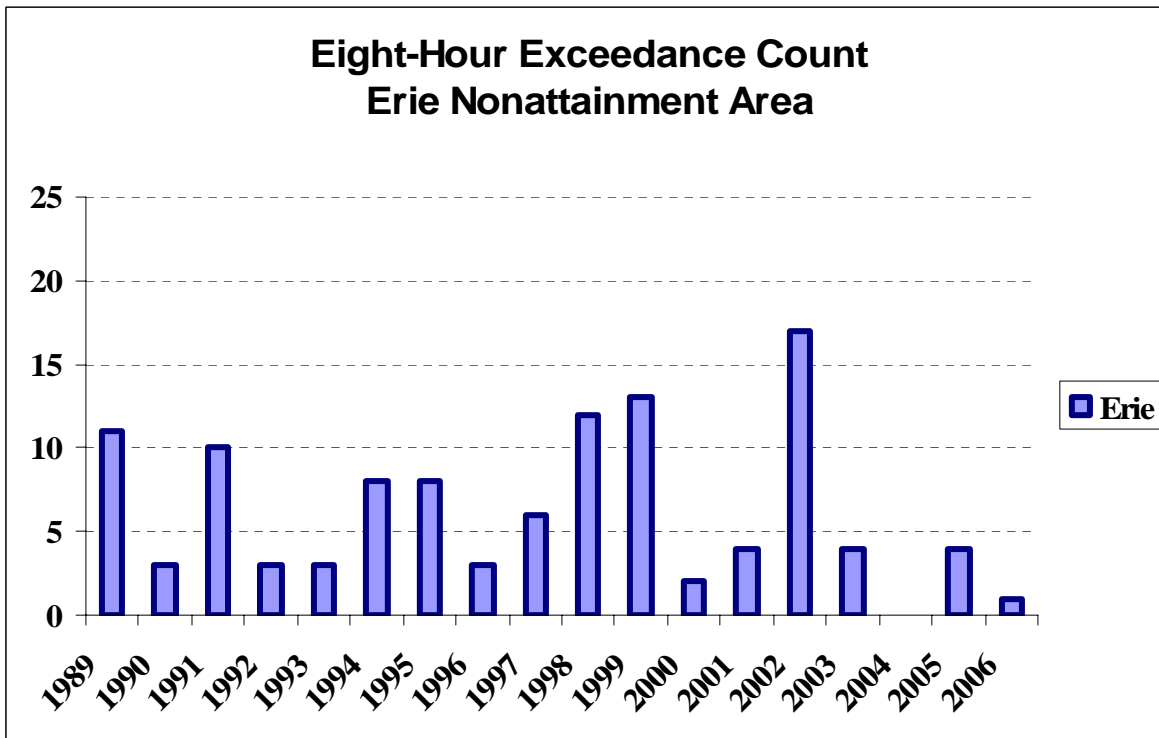
Chart 1-2 Exceedance Day Count for the Erie County Nonattainment Area
