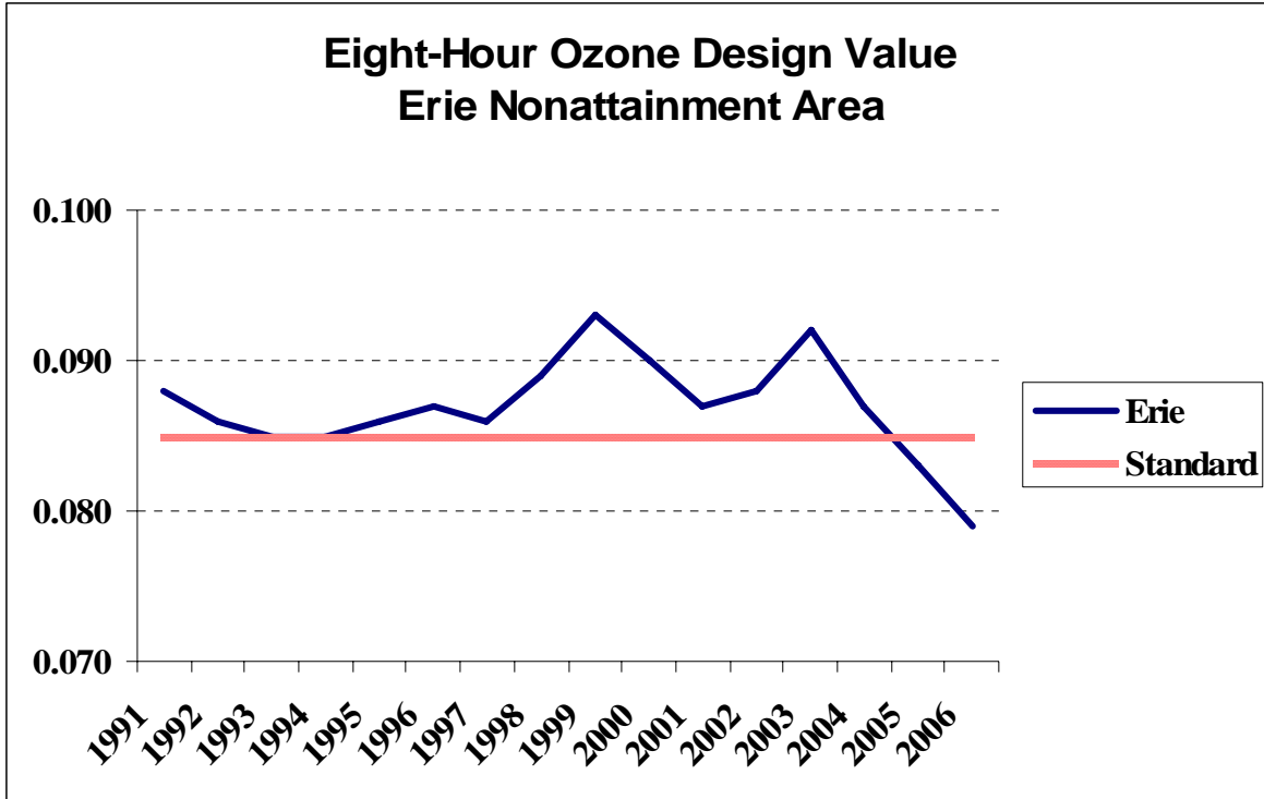
Chart 1-1 Eight-Hour Ozone Design Values
