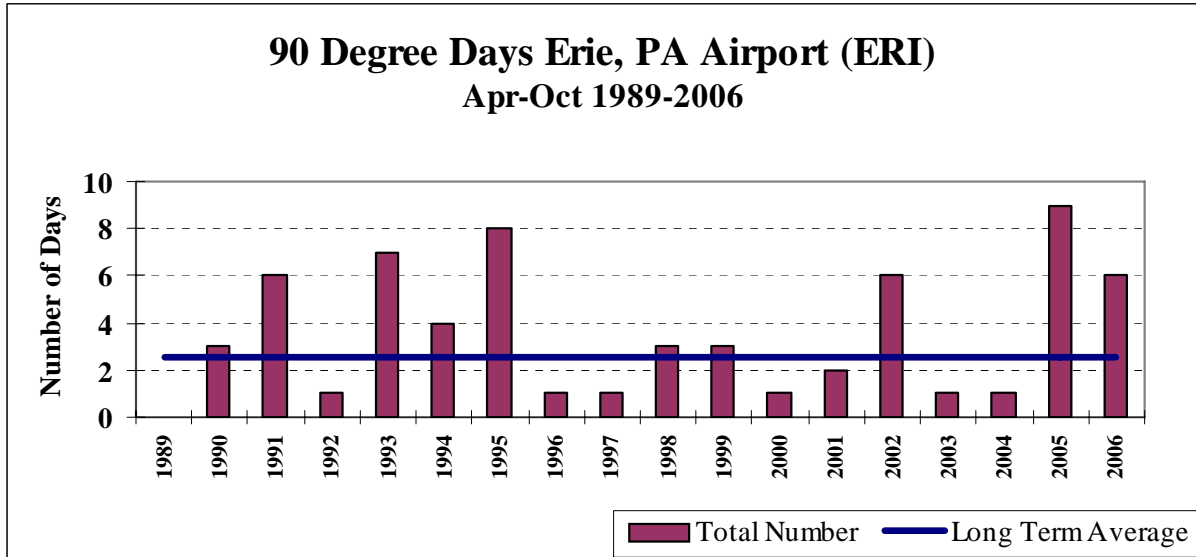
Chart 1-6 Number of 90° Degree Days at Erie
