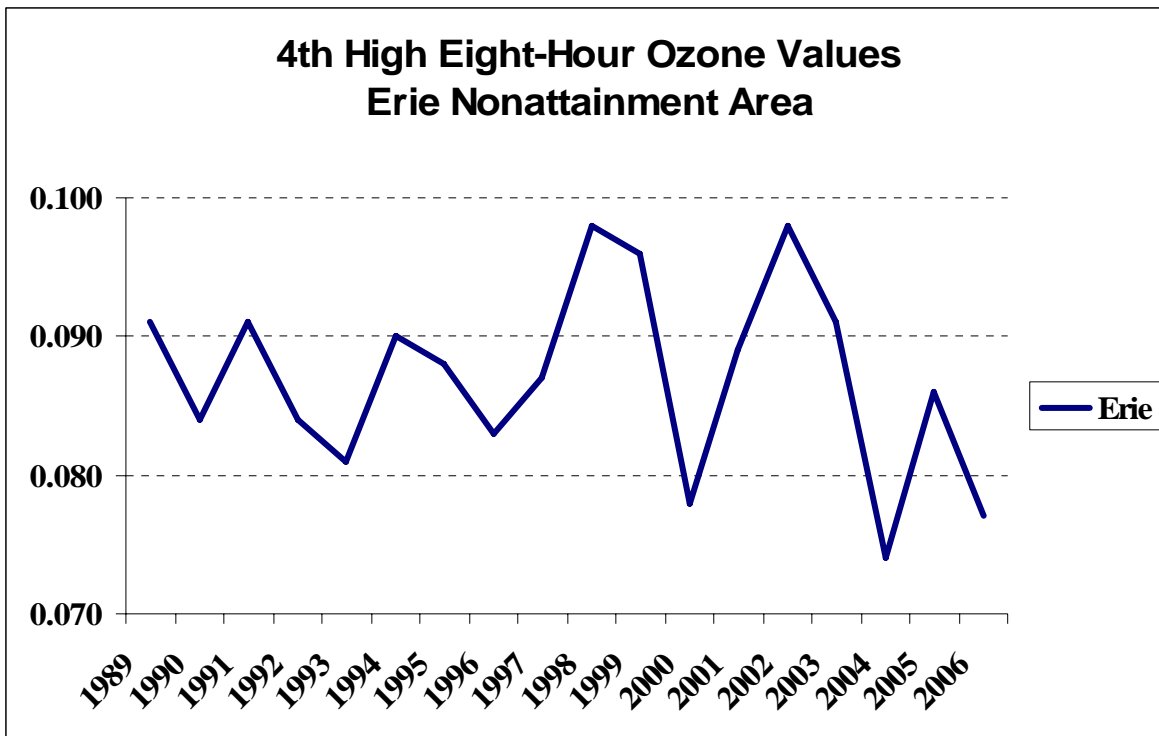
Chart 1-3 4 th High Eight-Hour Ozone Values for the Erie County Nonattainment Area
