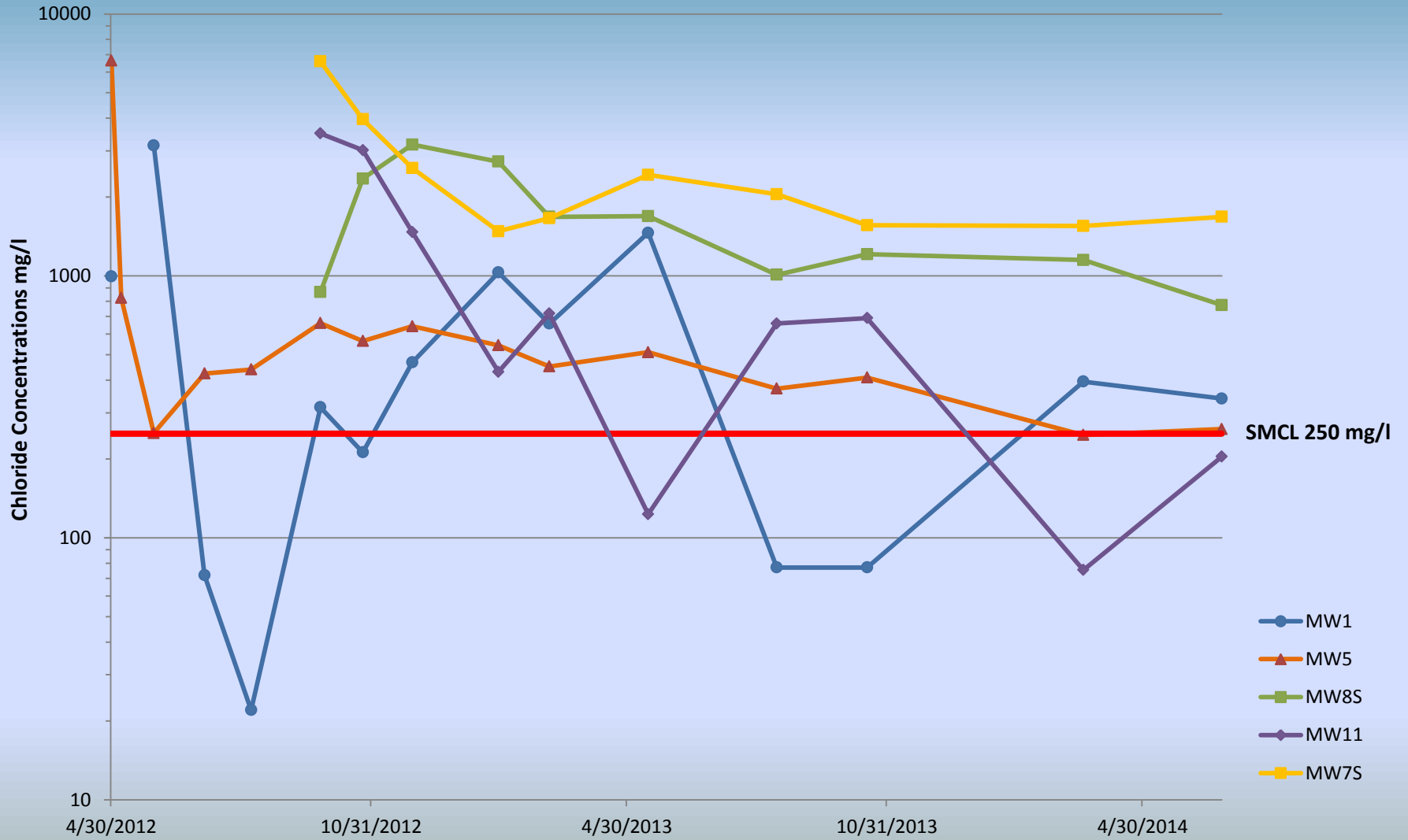
Exhibit H: Chloride concentrations versus time in select wells.
