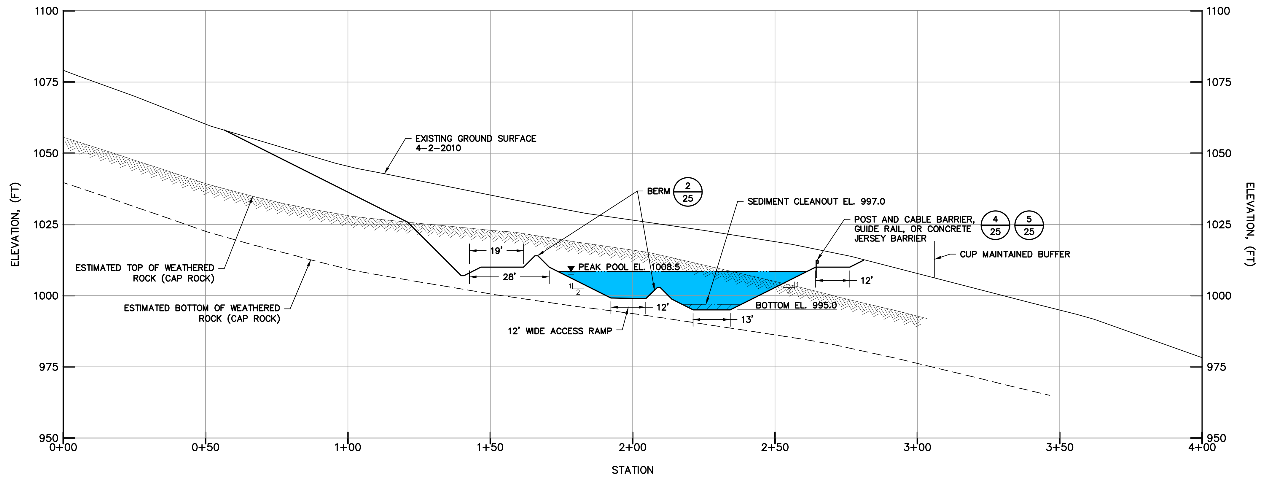
NT POND NO. 2 - SECTION A-A
