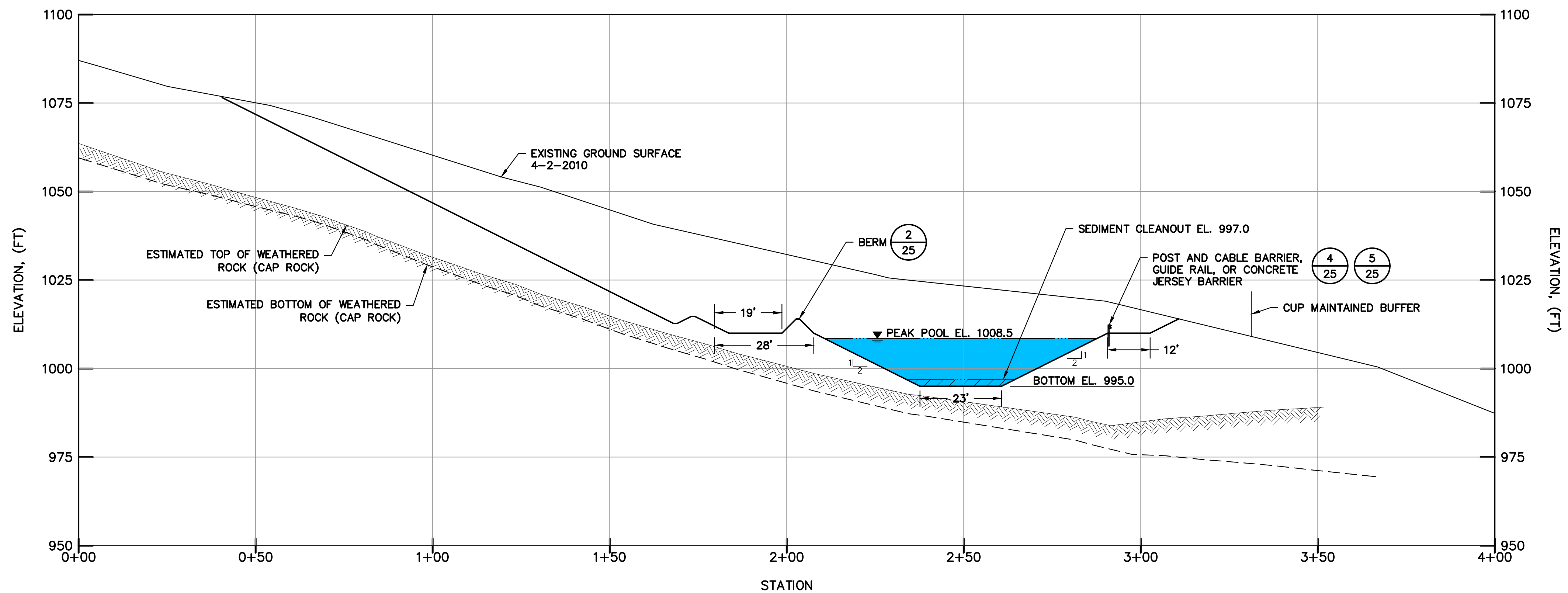
NT POND NO. 2 - SECTION B-B
