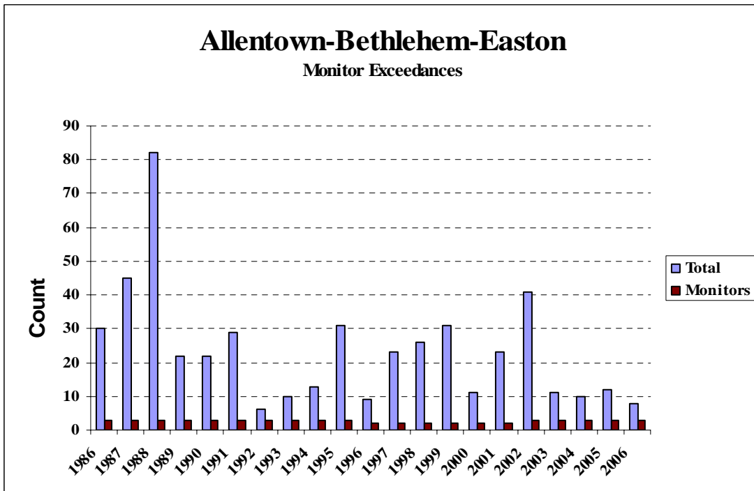
Chart 1-2 Monitor Exceedance Count for the Allentown Ozone Nonattainment Area
