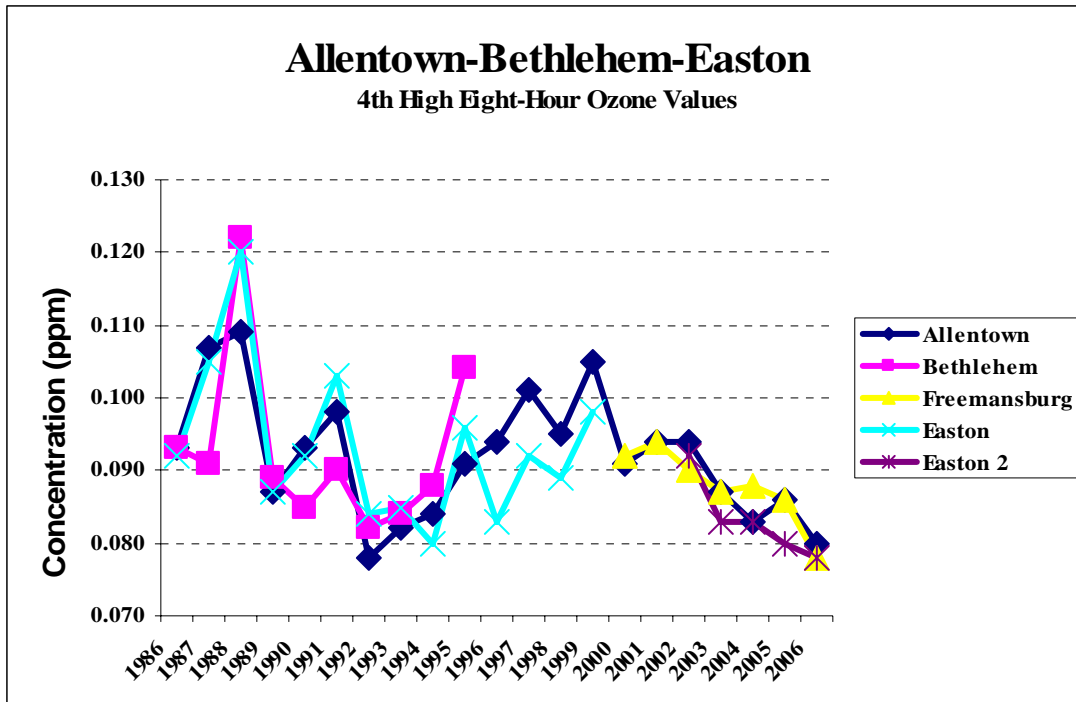
Chart 1-3 4 th High Eight-Hour Ozone Values for the Allentown Ozone Nonattainment Area
