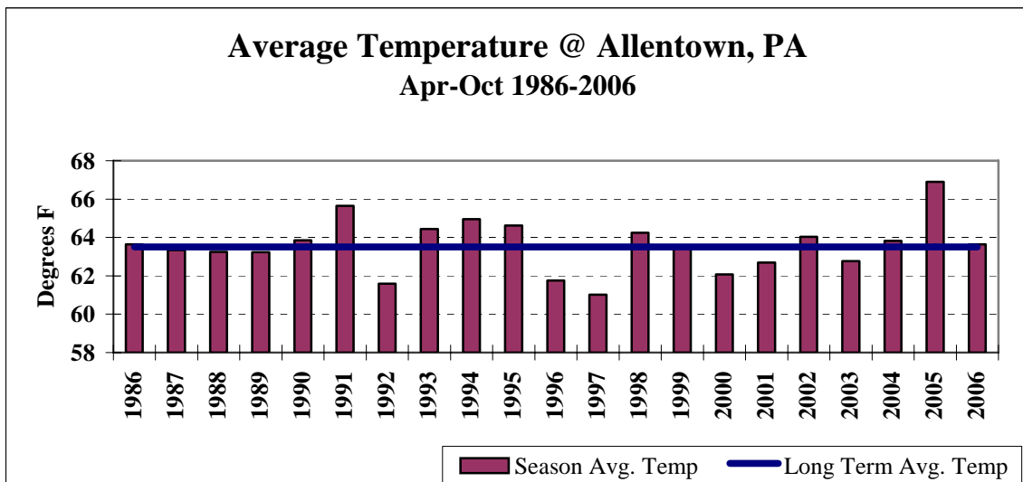
Chart 1-5 Average Temperatures at Allentown
