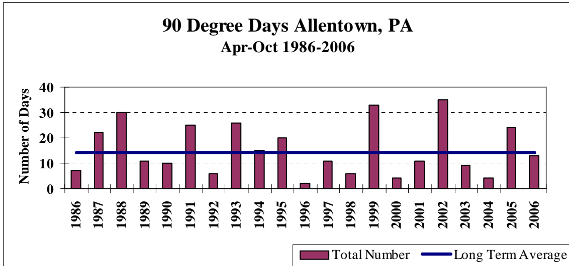
Chart 1-6 Number of 90° Degree Days at Allentown
