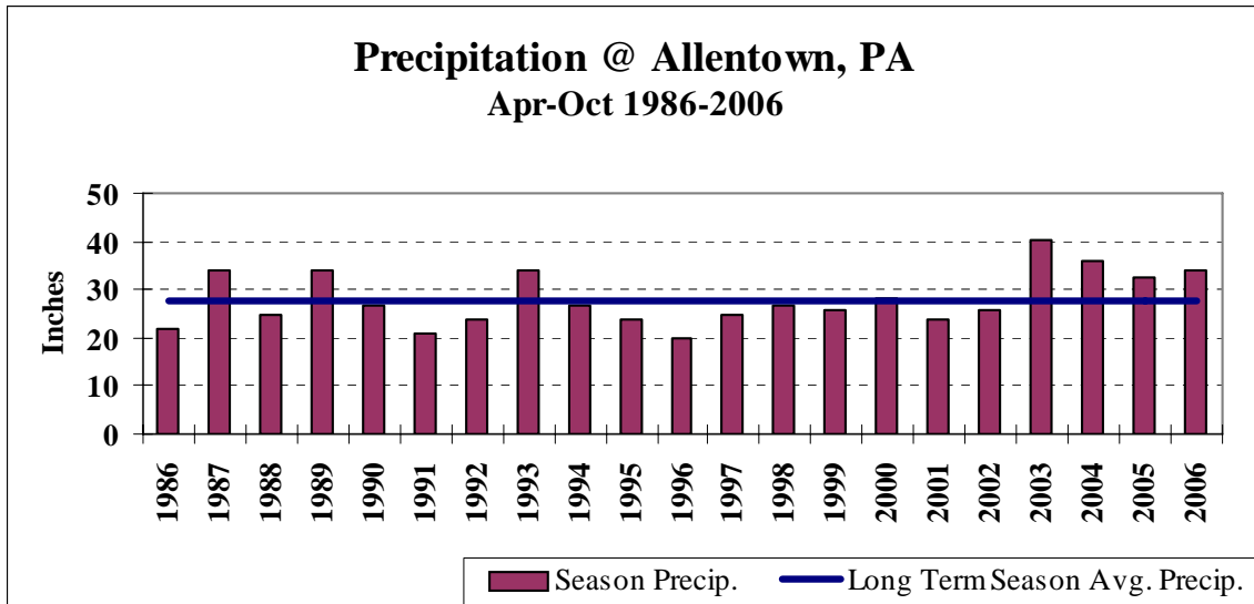
Chart 1-7 Precipitation Totals (inches) at Allentown
