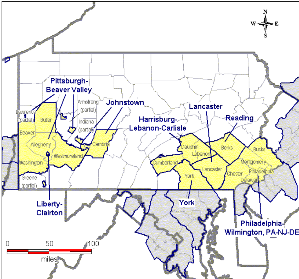
Figure 1-1 Harrisburg-Lebanon-Carlisle Annual PM 2.5 Nonattainment Area
