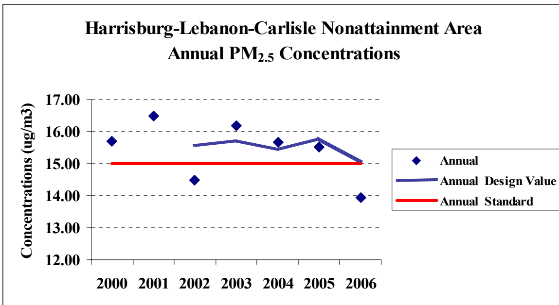
Figure 1-2 Annual Design Values: Harrisburg-Lebanon-Carlisle Annual PM 2.5 Nonattainment Area
