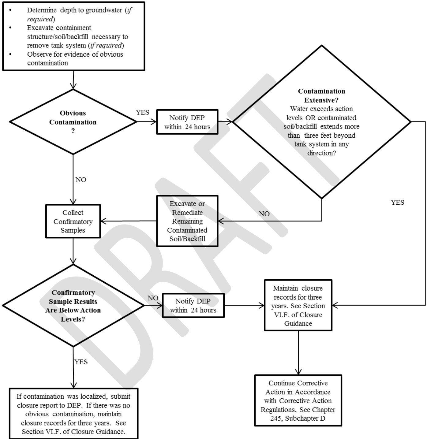
Figure 1 SITE ASSESSMENT Tank System Removal/Closure
