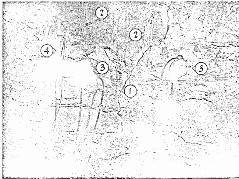
1. Crack caused by blasting. 2. Strain gauges. 3. Velocity transducers. 4. Accelerometer. Fig. 3—Stone basement wall showing typical transducer installation. Note that the crack produced by a test blast passes through two strain gauges
