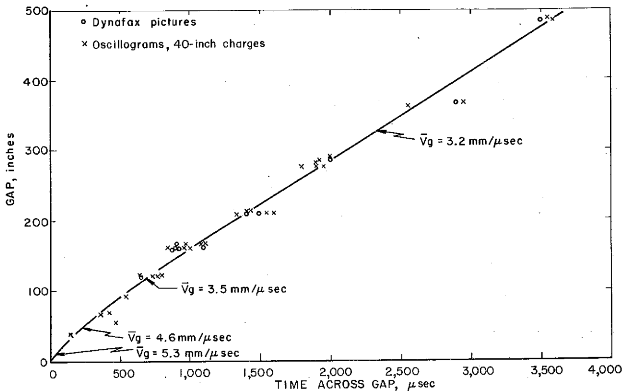
FIGURE 15. - Distance-Time Plot of Shock to Fragments Across Gaps for 40-Inch Donors.
