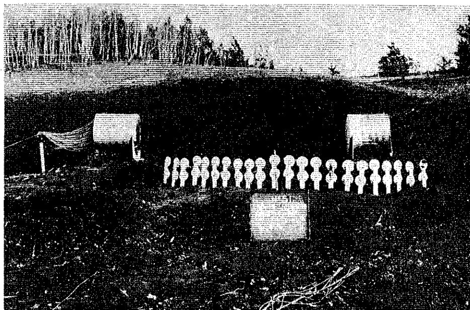
FIGURE 5. - Bank of Flashbulbs Used to Provide Supplemental Lighting for Dynafax Camera.
