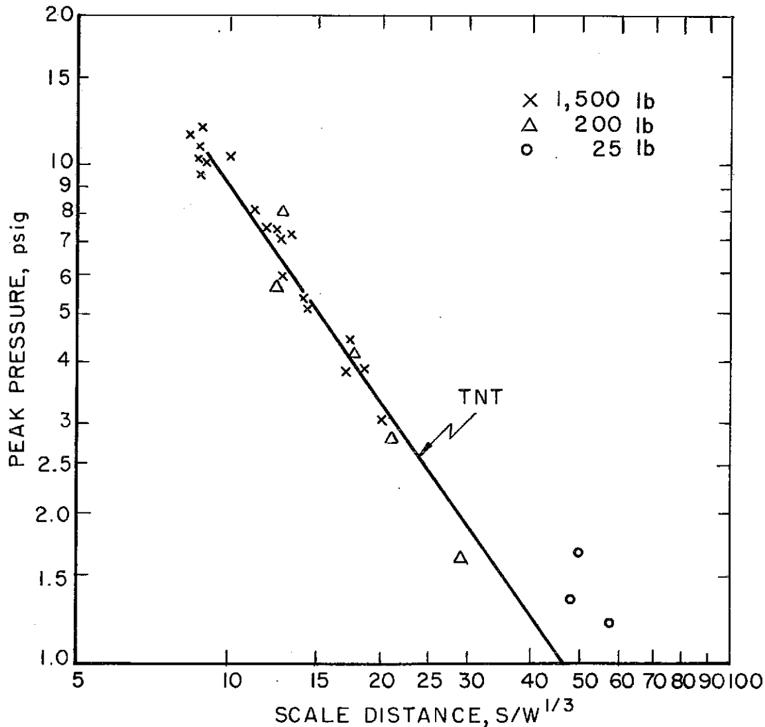
FIGURE 17. - Blast Pressures From AN-FO.
