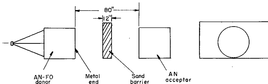
FIGURE 11. - Schematic of Charge-Sand Barrier Arrangement (Shot 59).
