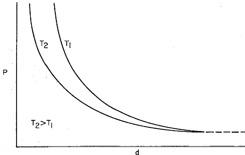
FIGURE 19. - Effects of Diameter ( d ) and Temperature ( T ) on Initiation Pressure ( P ).
