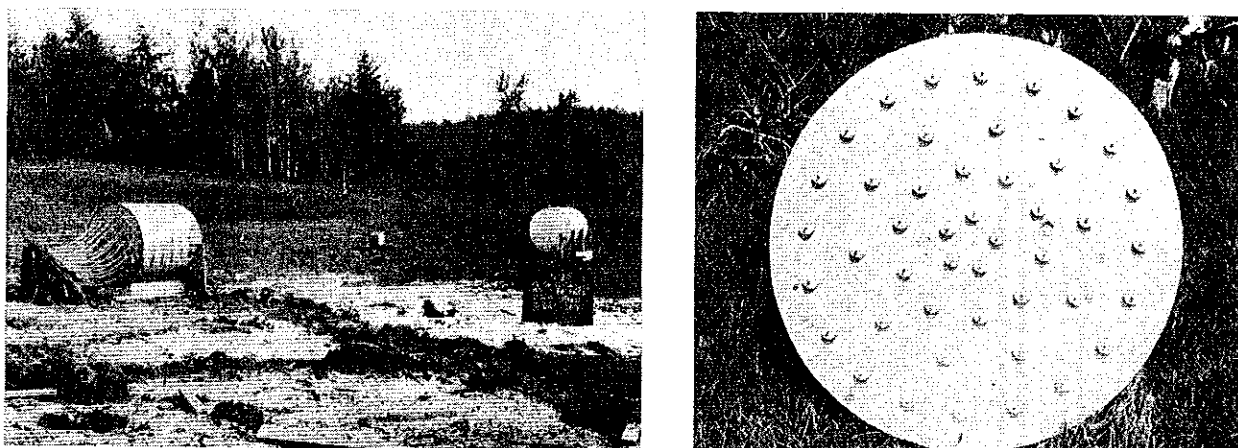
A B FIGURE 2. - (A) Donor and Acceptor in Place; Prills Seen in Foreground Are Result of a Previous Failure of the Acceptor To Be Initiated With a 10" x 10" Donor at Gap Distance of 30 Inches. (B) Donor Booster Showing Installation of RDX Pellets.
