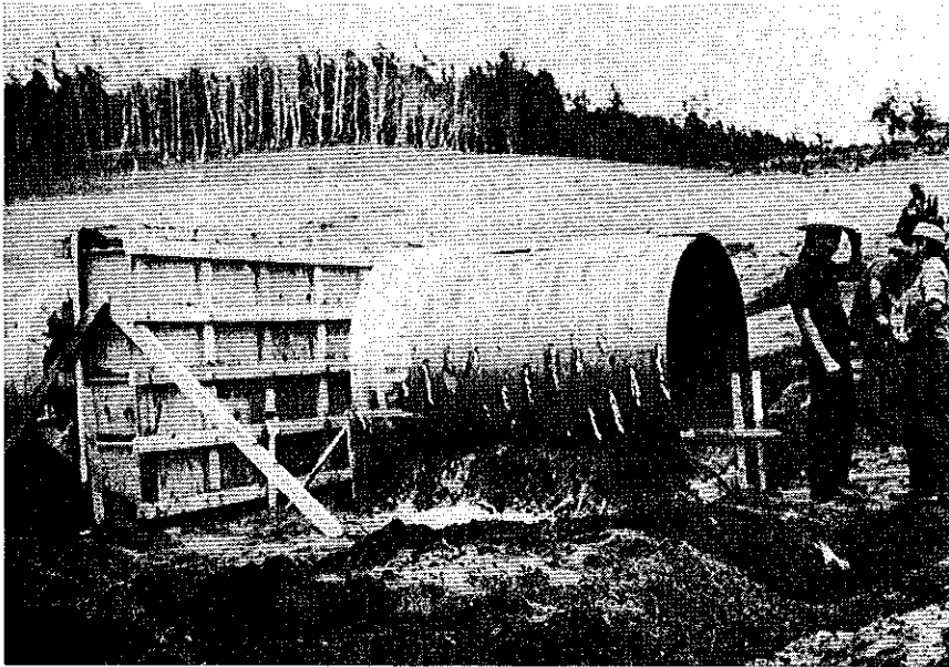
FIGURE 11. - Preparation of 60-Inch Barricade Shot.
