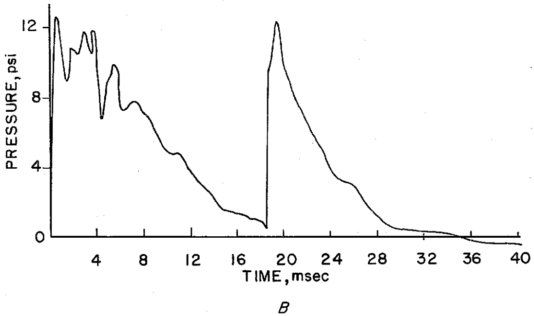
FIGURE 18. - Typical Airblast Pressure Profiles. A, 5,400-pound AN-FO donor at 110 feet; B, 1,600-pound AN-FO donor and AN-FO acceptor showing two separate blast waves.
