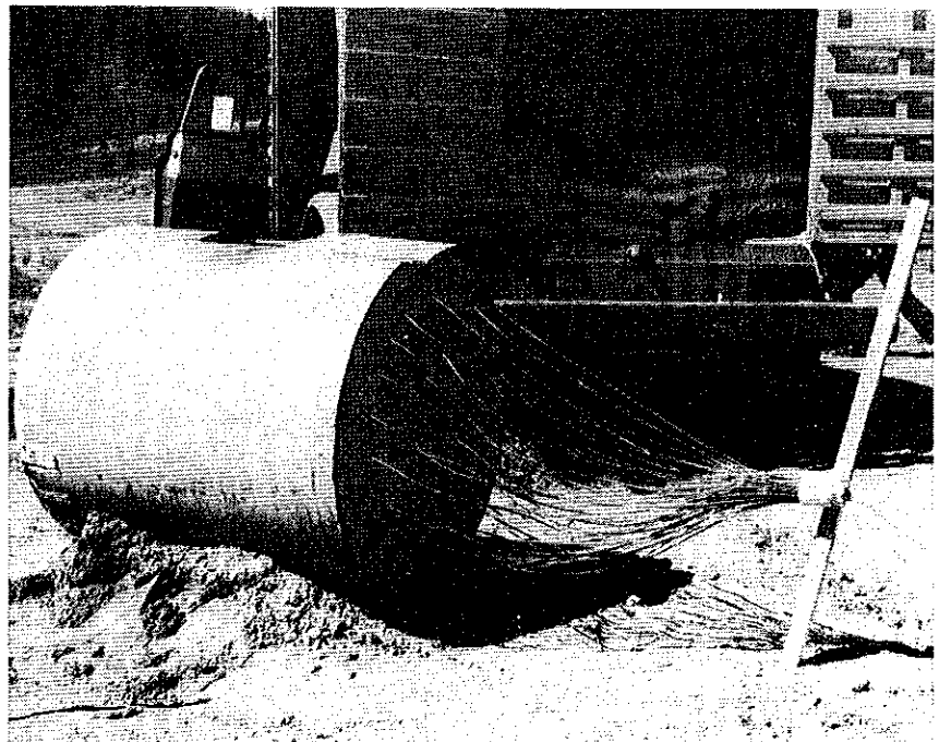
FIGURE 7. - Donor Charge Showing Multipoint Initiation System.
