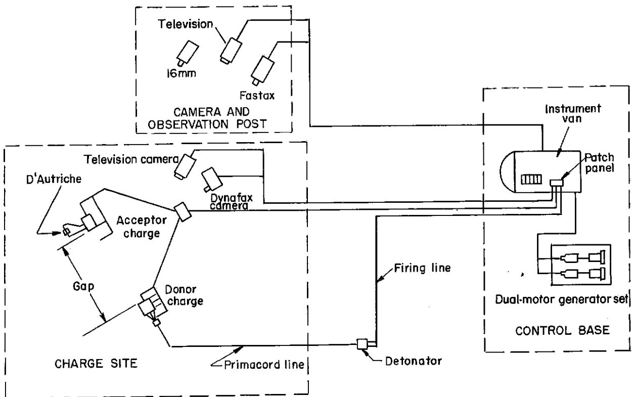
FIGURE 5. - Field Instrumentation.
