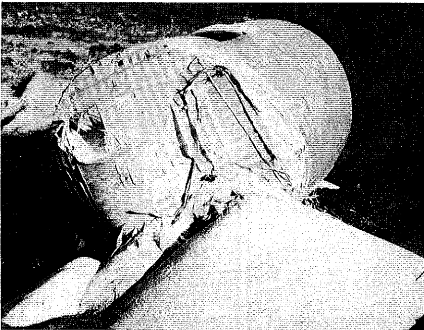
FIGURE 1. - Failure of 60-Inch AN-FO Acceptor Shot With Metal-Ended Donor at 182 Feet.
