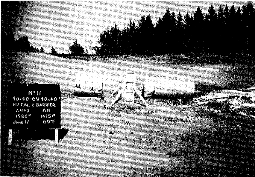
FIGURE 10. - Forty-Inch AN-FO and AN Charges Separated 5-2/3 Feet by a 10-Inch Barrier. Two failures in three shots occurred at this distance.
