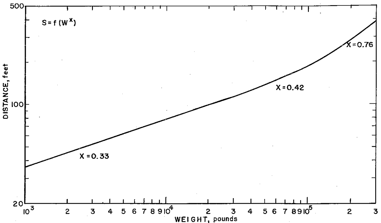
FIGURE 20. - Plot of American Table of Distances Showing Three Values of the Exponent in the Equation S = F(W^x) .
