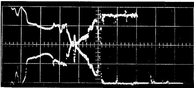
FIGURE 22. - Oscillograms for Continuous Probes for Detonation Velocity. A, Stable detonation in 60-inch AN-FO donor; B, delayed initiation and unstable detonation in bagged AN-FO.
