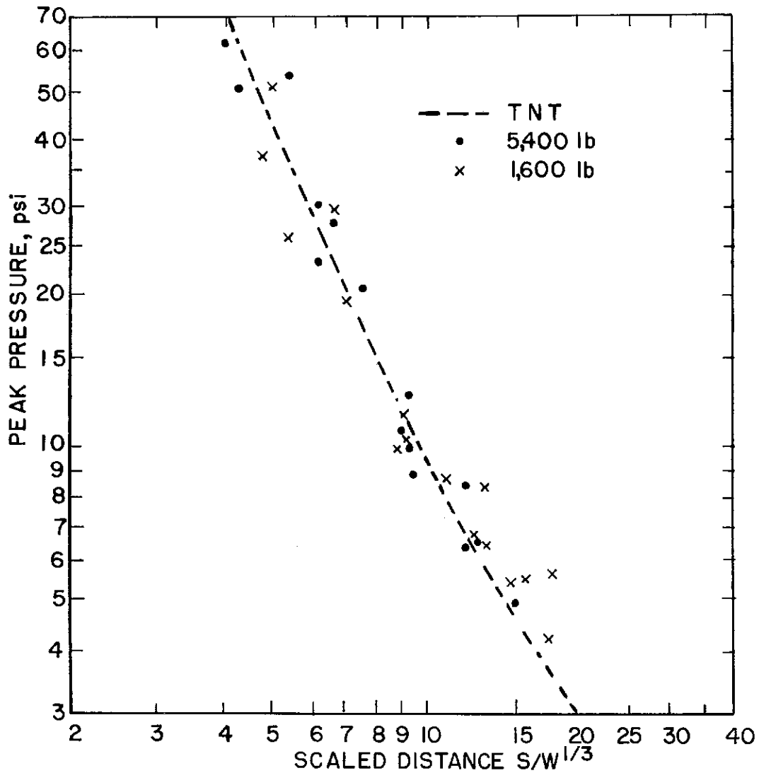
FIGURE 19. - Peak Pressure Versus Scaled Distance for AN-FO Compared With TNT.
