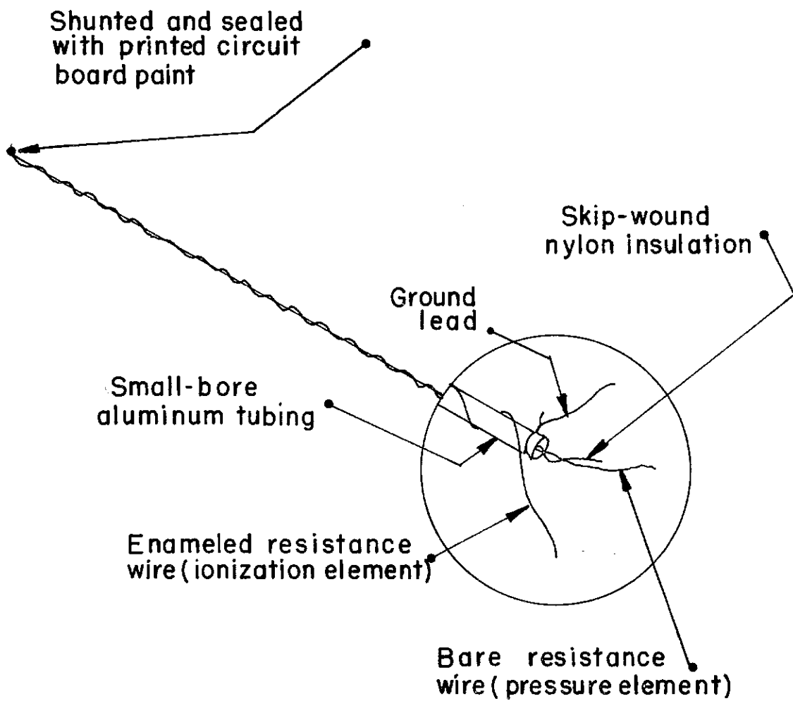
FIGURE 4. - Concentric Probe for Measuring Detonation Velocities.
