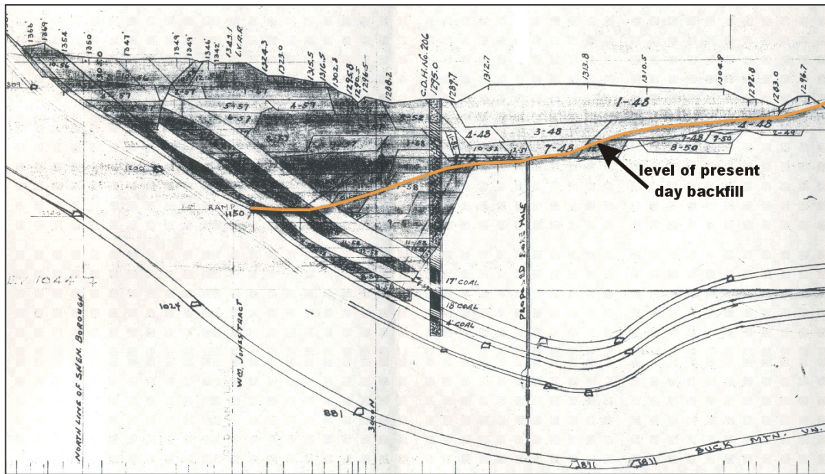
Figure 7.4. Cross-section through Shen Penn Pit (48+00E) showing surface mining locations and dates.
