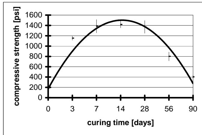
Figure 7.11. Strength development in lime kiln dust (LKD) activated fly ash grout as a function of curing time.
