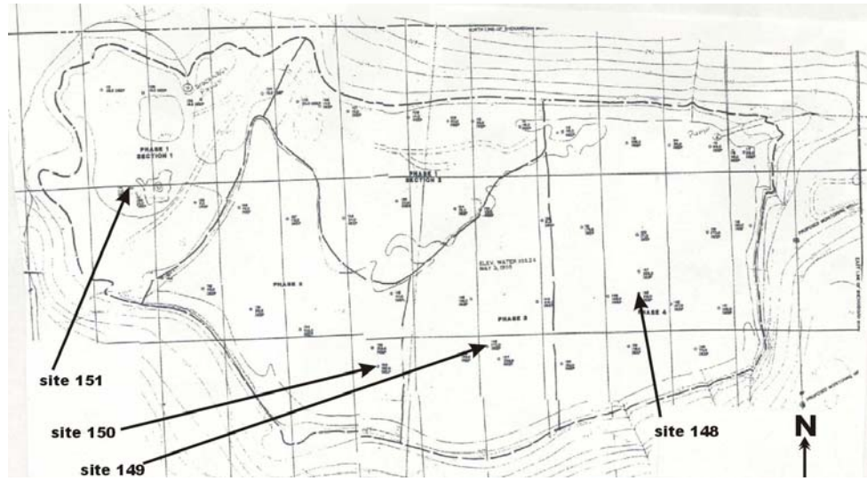
Figure 7.6. Shen Penn site map with locations of chemical sampling. The area of open connection to the deep underground mine is to the southeast.
