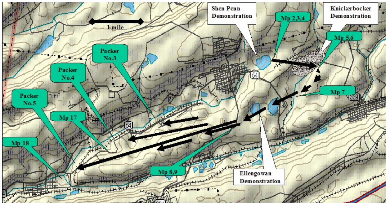
Figure 7.5. Projected flow path from minepool water discharging from the vicinity of the Shen Penn demonstration site (Laslow, pers. Communication, 2004). (Mp's are relevant DEP monitoring points utilized to establish mine pool flow pattern.)
