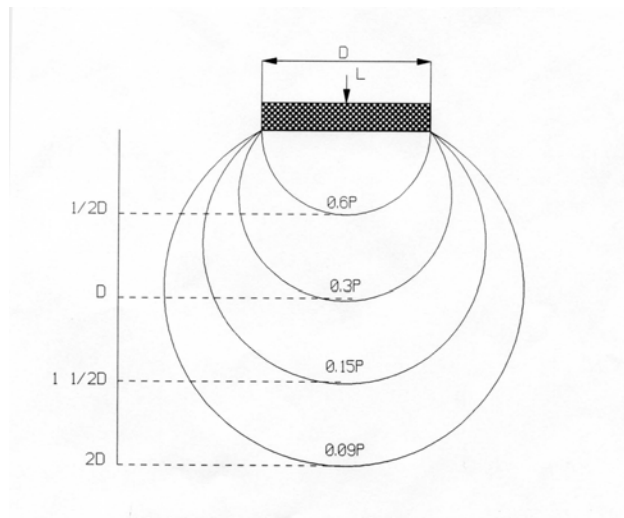
Figure 7.14. Variation in compaction pressure with depth under a load.
