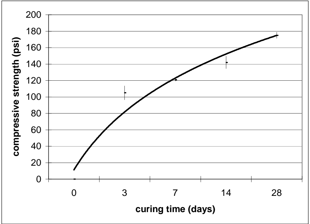
Figure 7.13. Strength development in CKD activated fly ash grout as a function of curing time.
