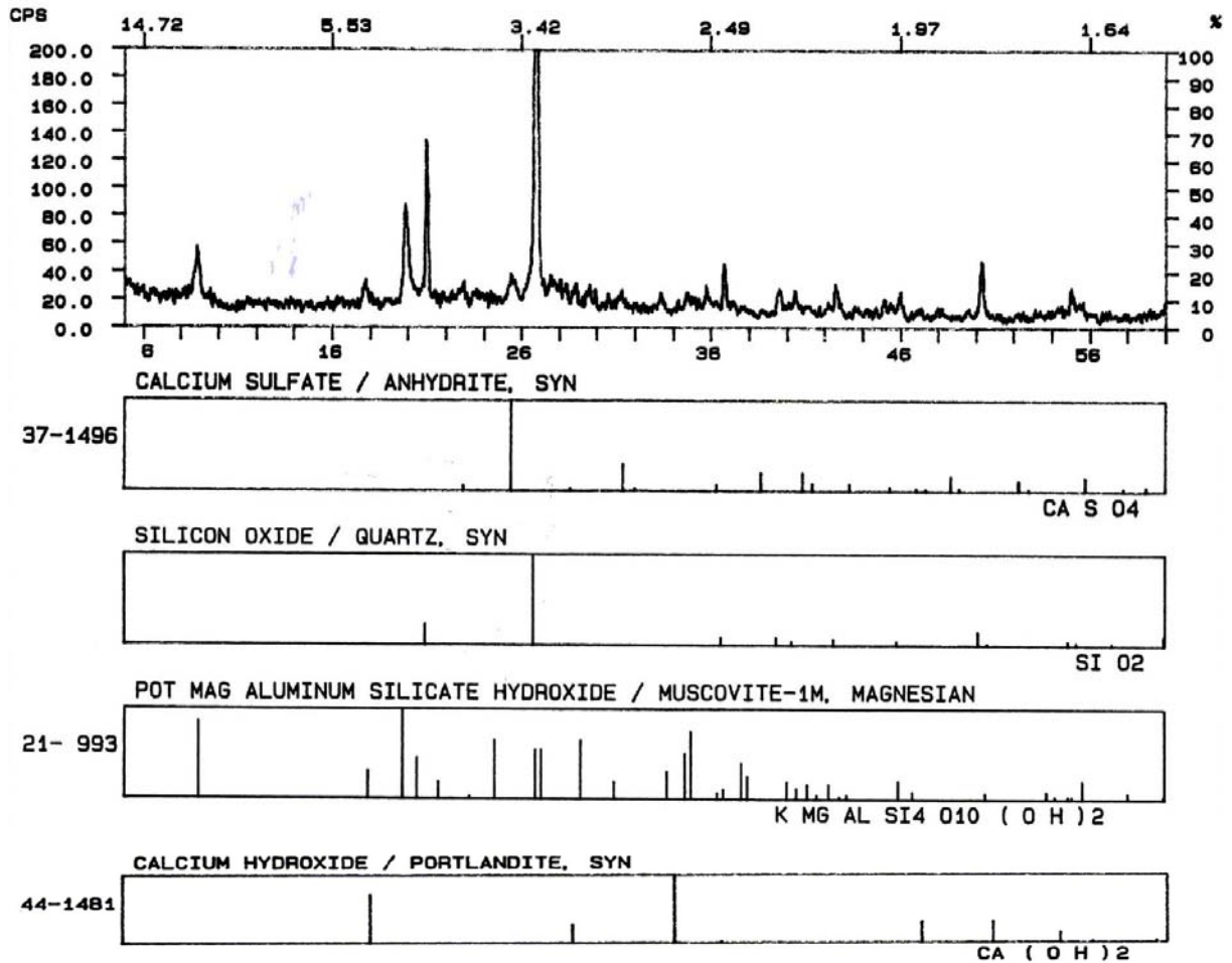
Figure 7.7. X-ray diffraction pattern and identified crystalline phases present in SER bottom ash.
