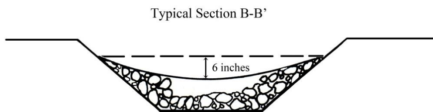
Figure 2.5. Rock Filters
