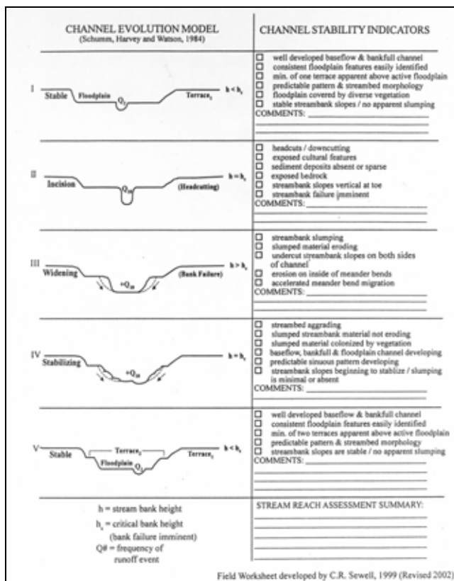
Figure 3. Channel Evolution Model (Schumm, Harvey and Watson 1984; field observation checklist adapted by Randy Sewell, VHB, Inc., Williamsburg, VA)
