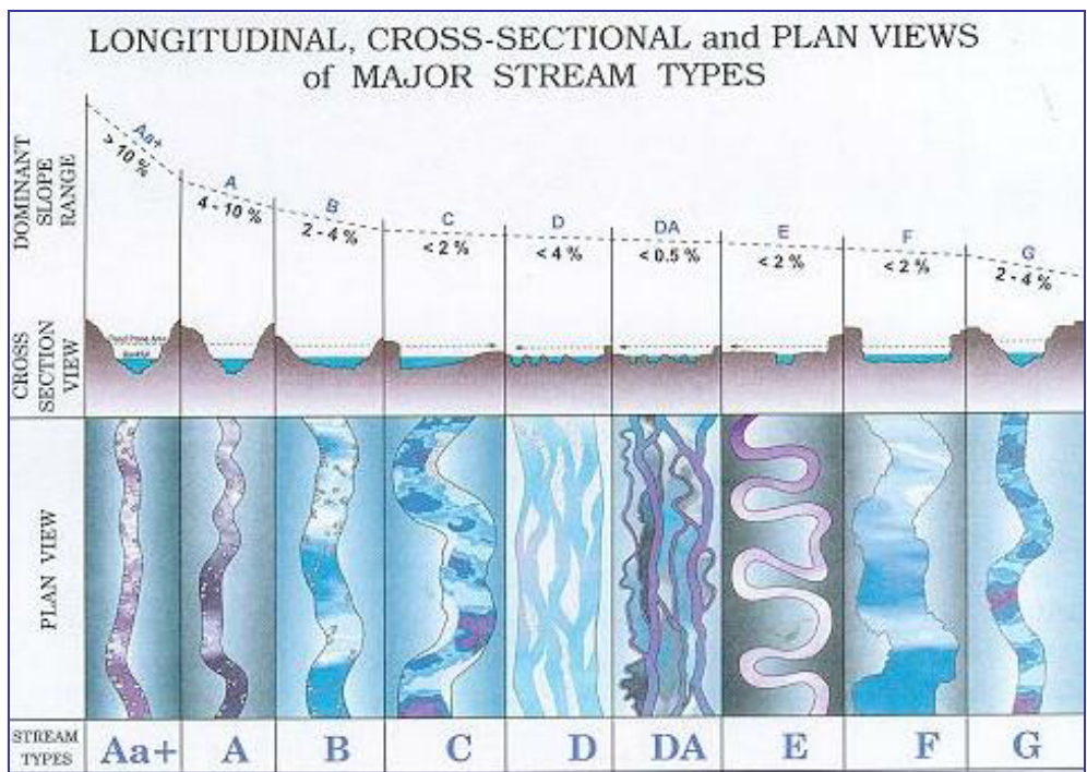
Figure 2. Stream types (from Rosgen 1994, 1996).
