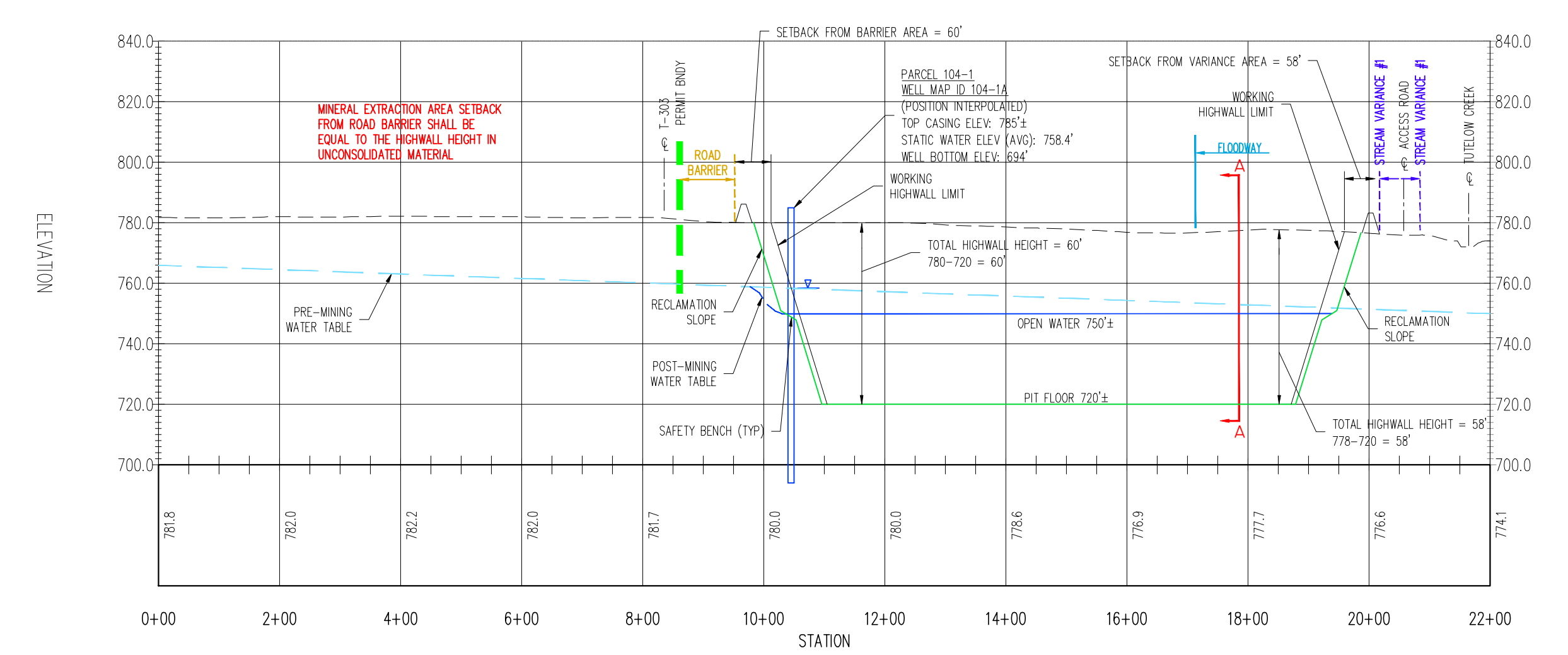
Section E-E'
