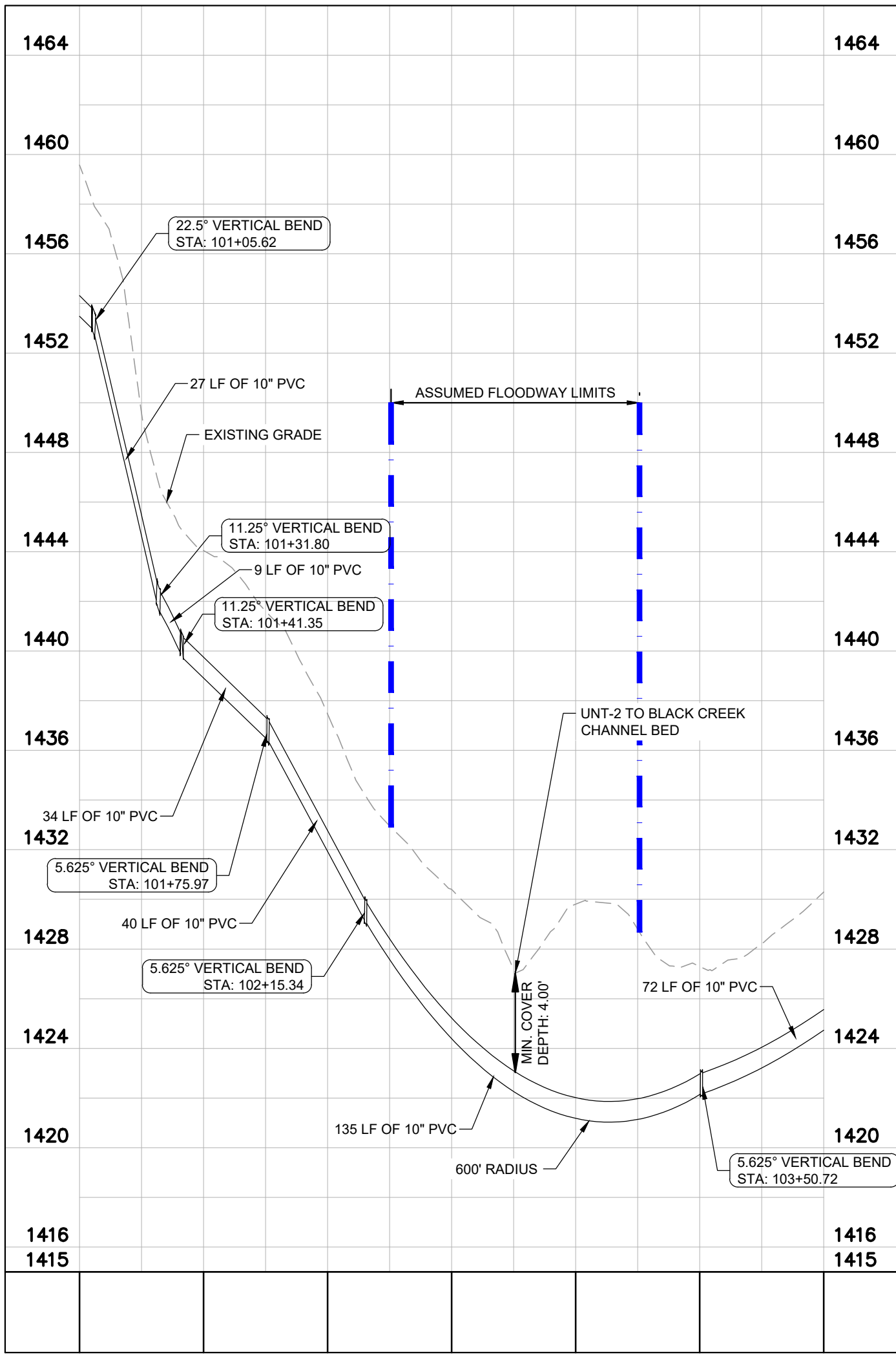
IRRIGATION ALIGNMENT SCALE 1" = 50' H 1" = 5' V
