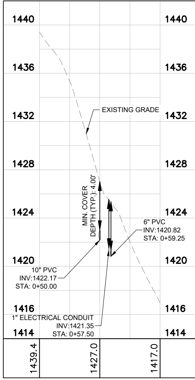
CHANNEL CENTERLINE SCALE 1" = 50' H 1" = 5' V
