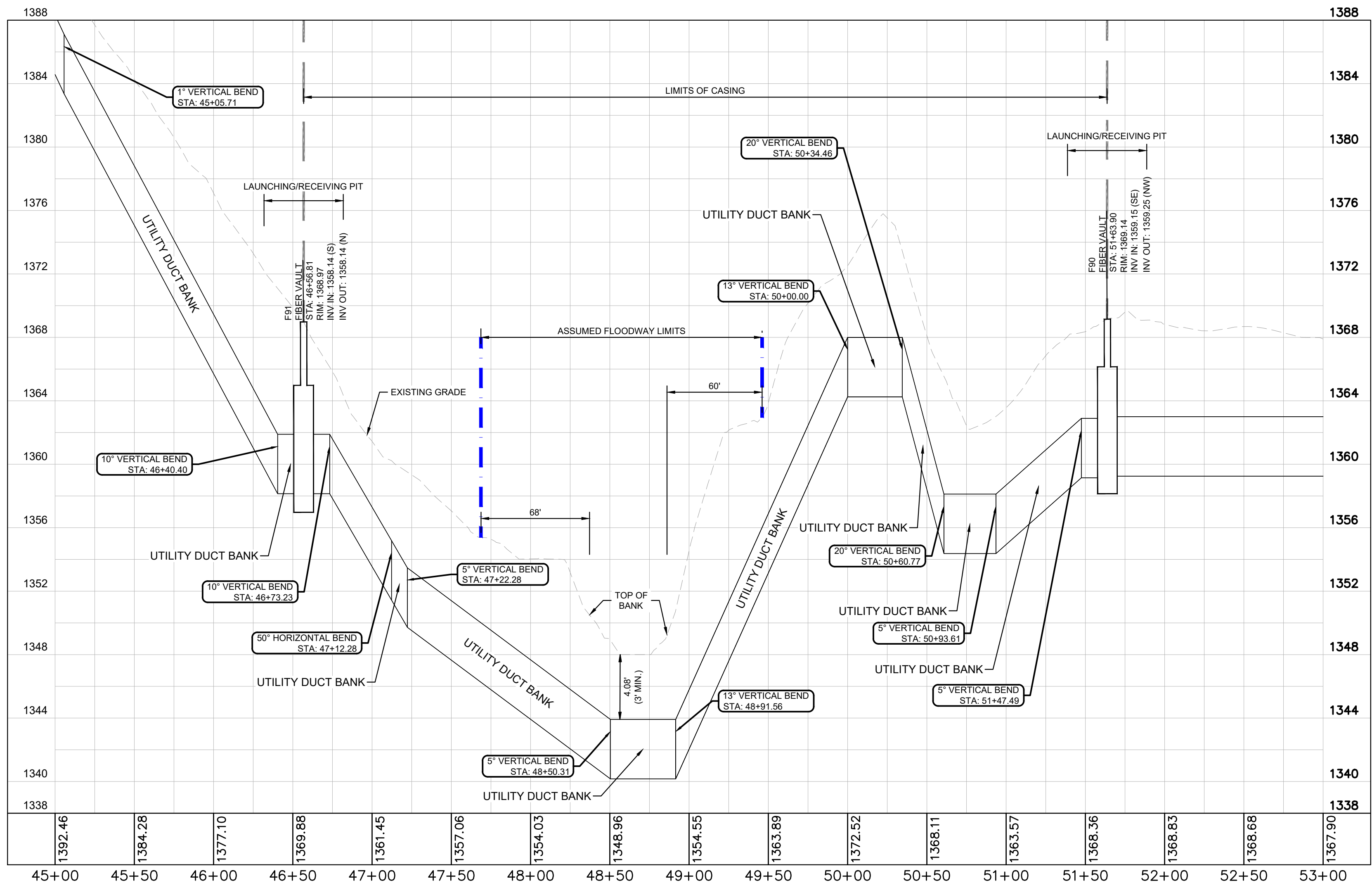
FIBER 11 SCALE 1" = 50' H 1" = 5' V
