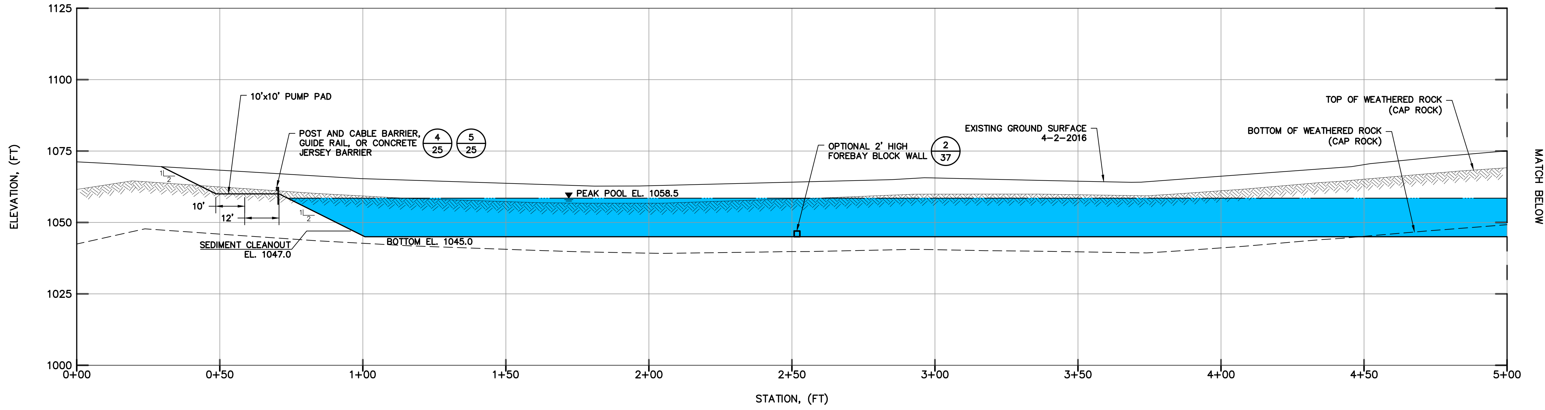
NT POND NO. 1 - SECTION D-D
