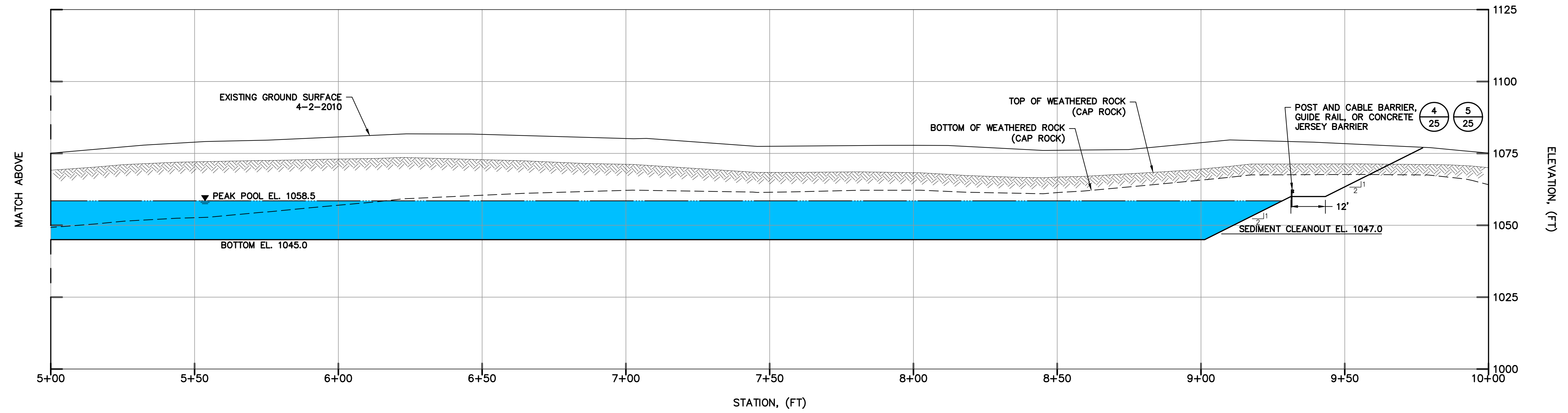
NT POND NO. 1 - SECTION D-D (CONTINUED)
