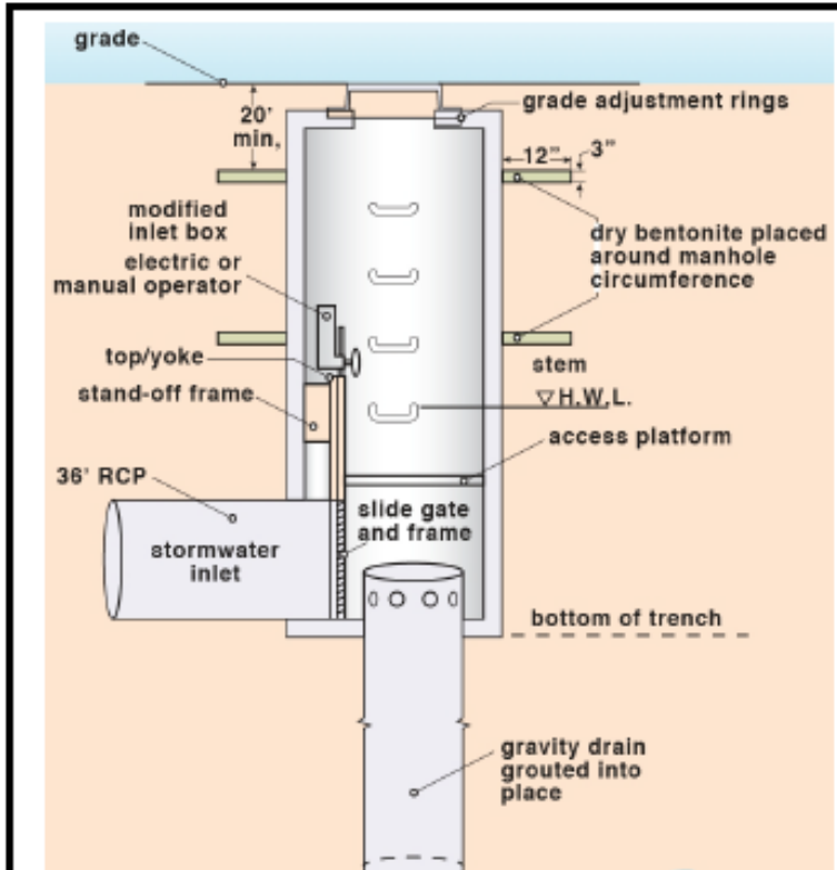
Figure 3. Injection well manhole design
