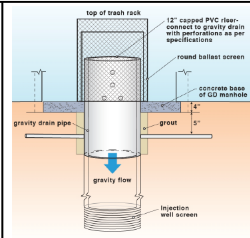
Figure 4. Gravity drain flow restrictor
