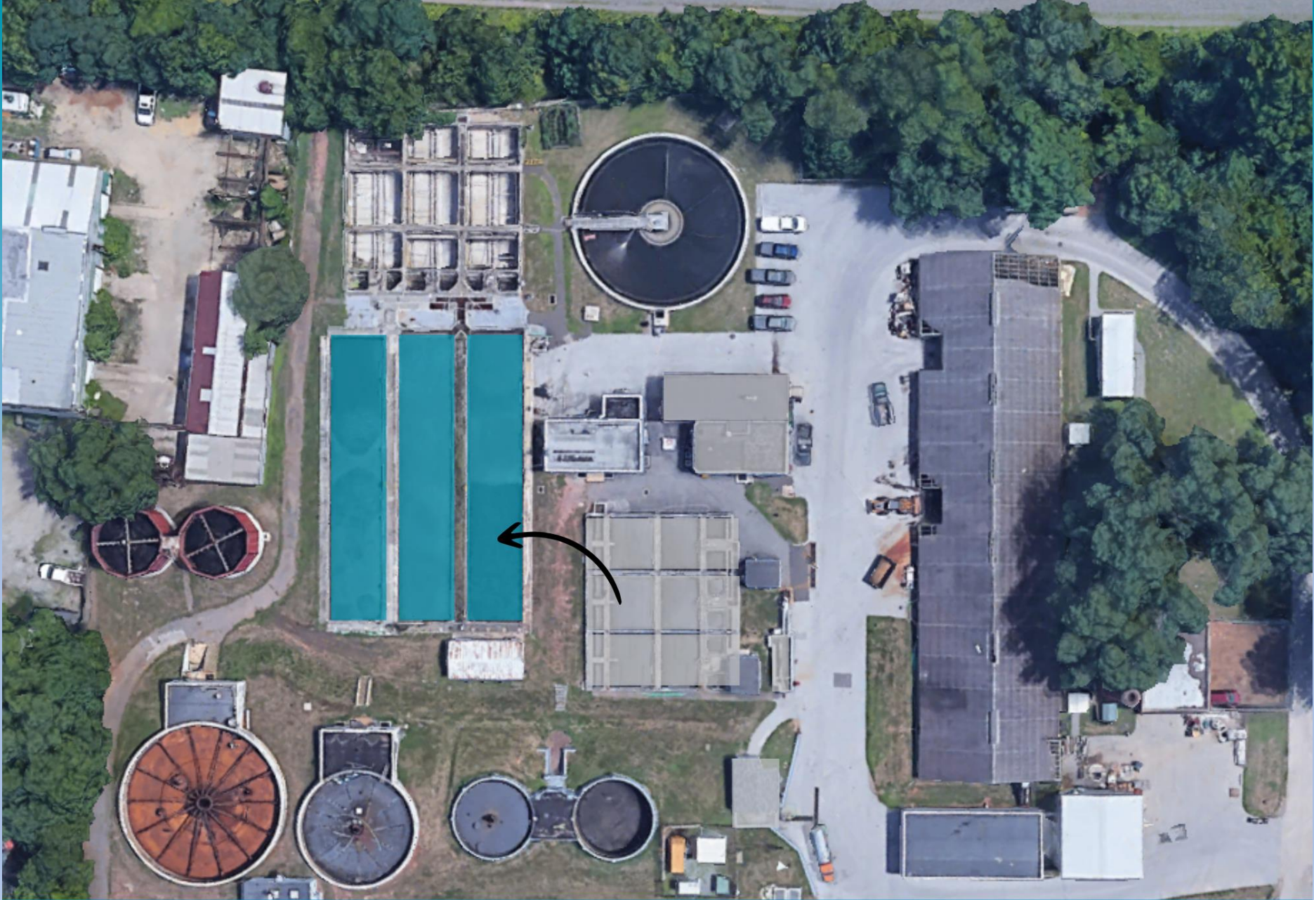
AERATION TANKS
