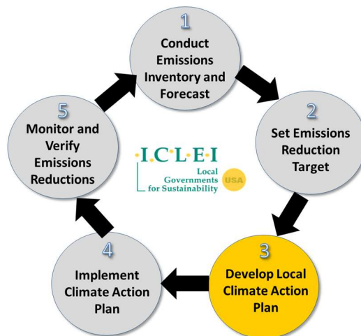
Figure 1: Five Milestones for Climate Mitigation
