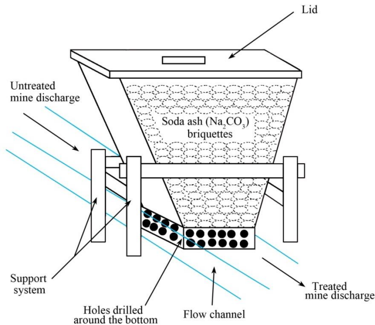
Figure 6.2. Typical Neutralizing Unit
