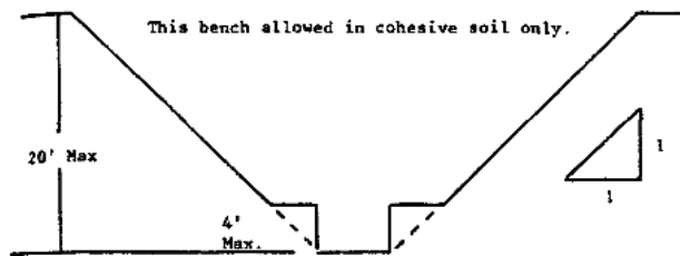
SINGLE BENCH
