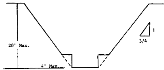
SIMPLE BENCH
