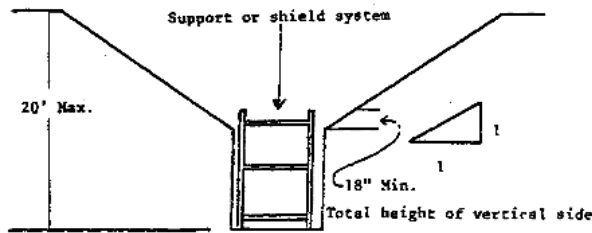
VERTICALLY SIDED LOWER PORTION
