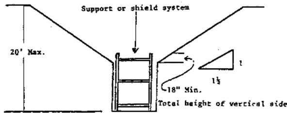
VERTICAL SIDED LOWER PORTION
