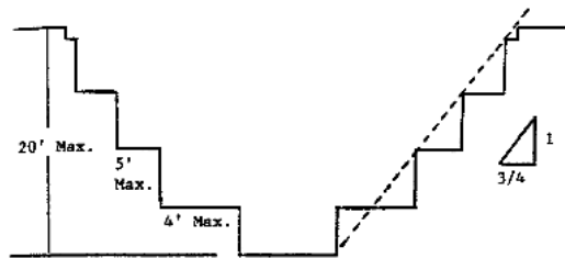
MULTIPLE BENCH
