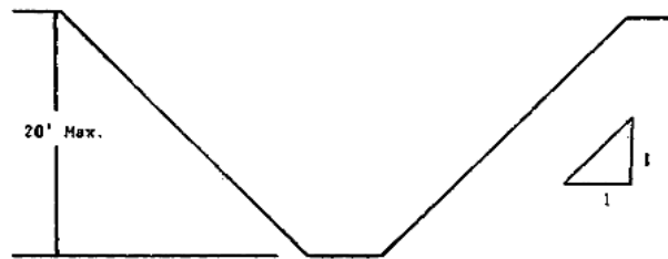
SIMPLE SLOPE
