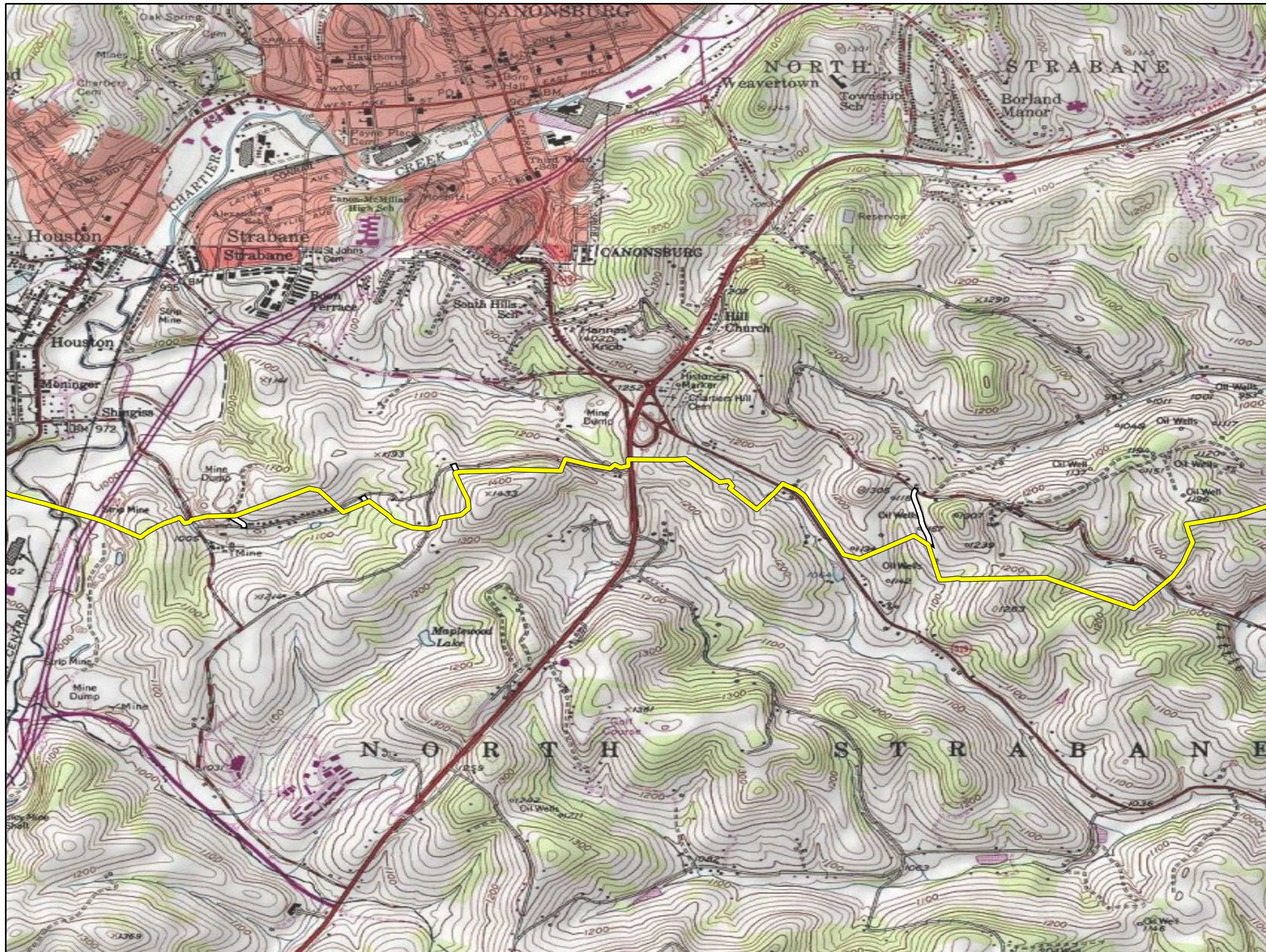
Figure 1. Project Location for the Sunoco Pennsylvania Pipeline Project, Washington County, PA. Sheet 2 of 5
