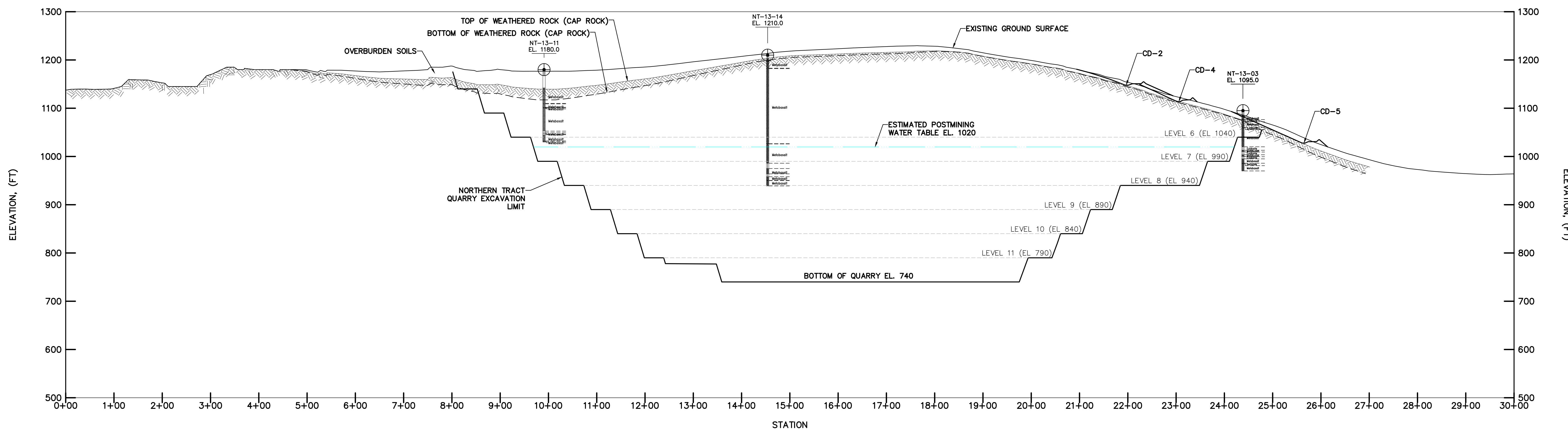
GEOLOGIC SECTION B-B
