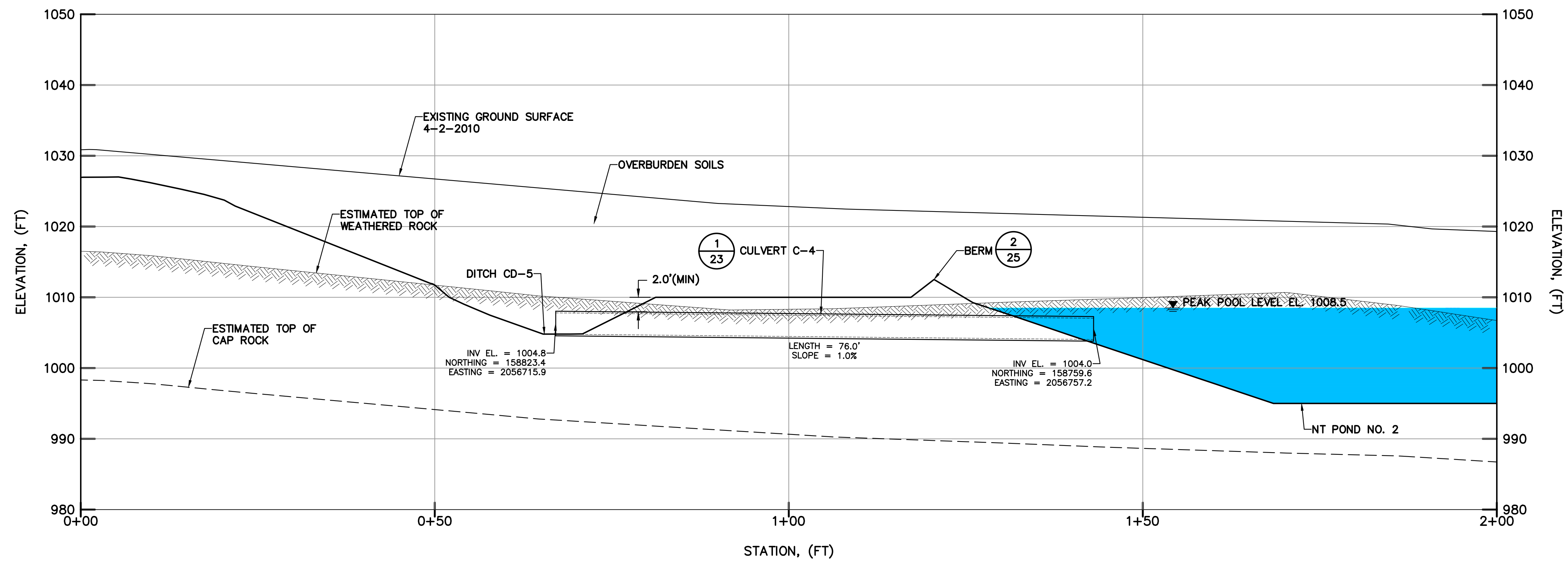
SECTION A-A (CULVERT C-4)
