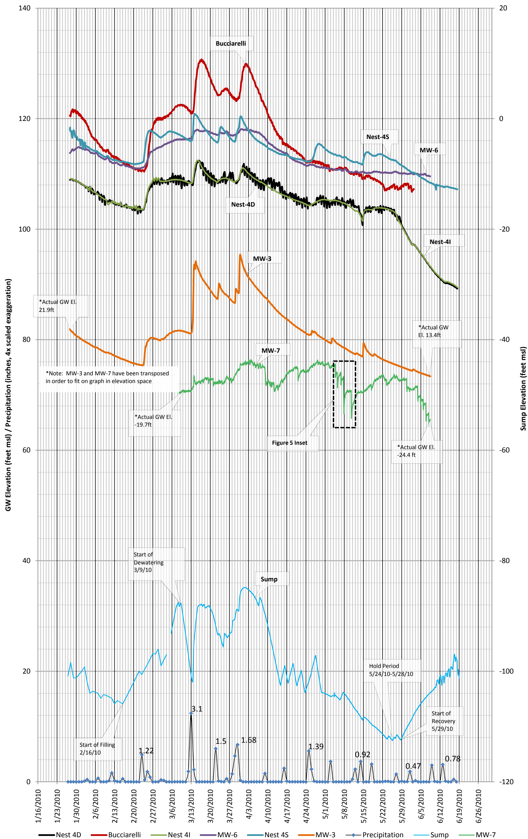
Figure 4. Monitoring Wells and Sump Hydrograph
