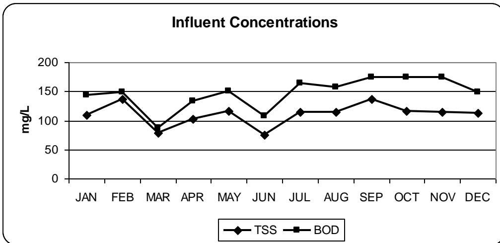
Figure 2.1 Graph of Influent Concentrations Showing Trends
