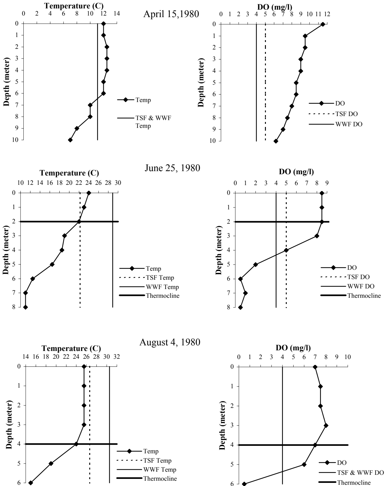
FIGURE 2. WALKER LAKE - WATER CHEMISTRY - Temperature and Dissolved Oxygen Profiles Ulanoski and Shertzer 1981 Vertical lines depict parameter criteria.
