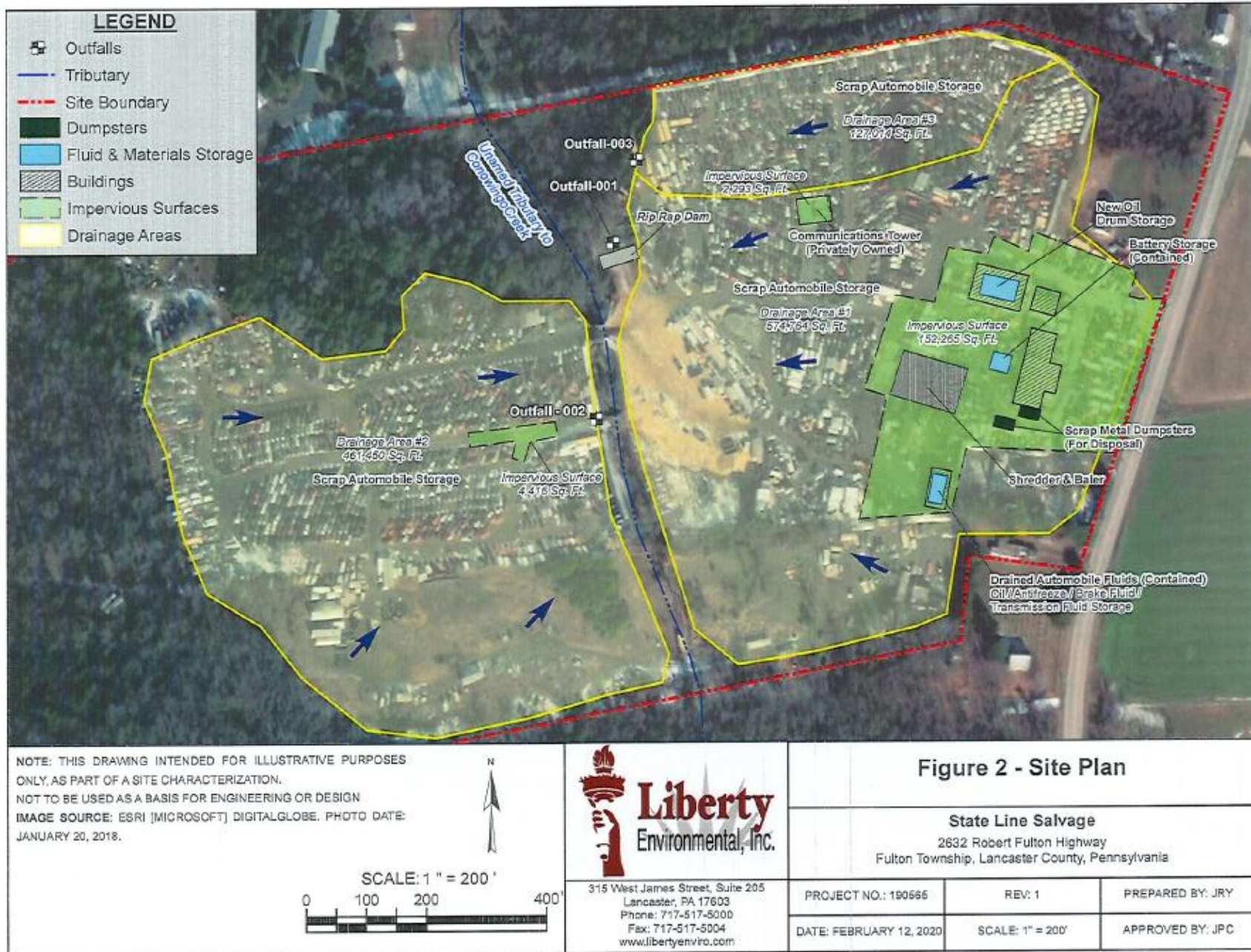
FIGURE 2. SITE PLAN
