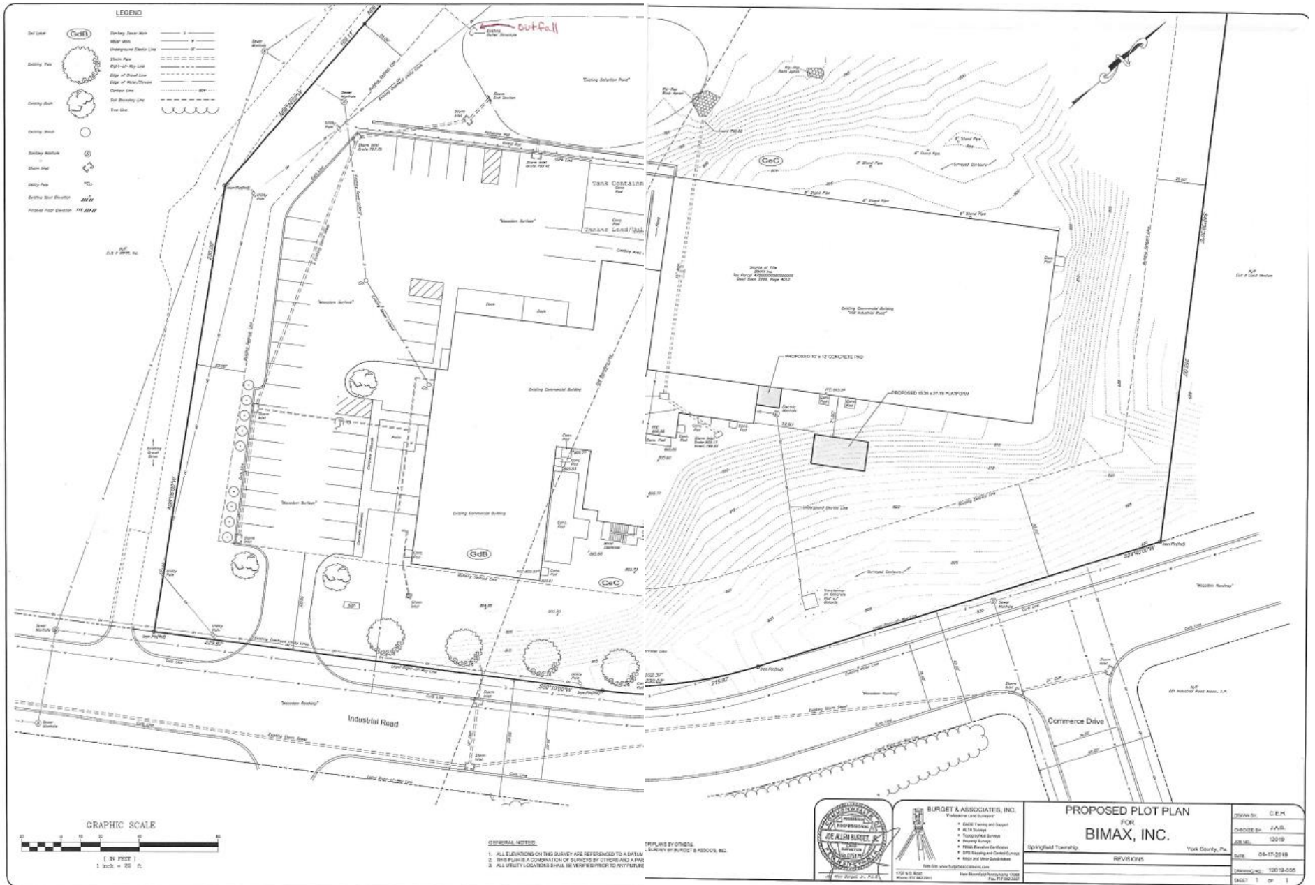
Figure 4. Facility Layout
