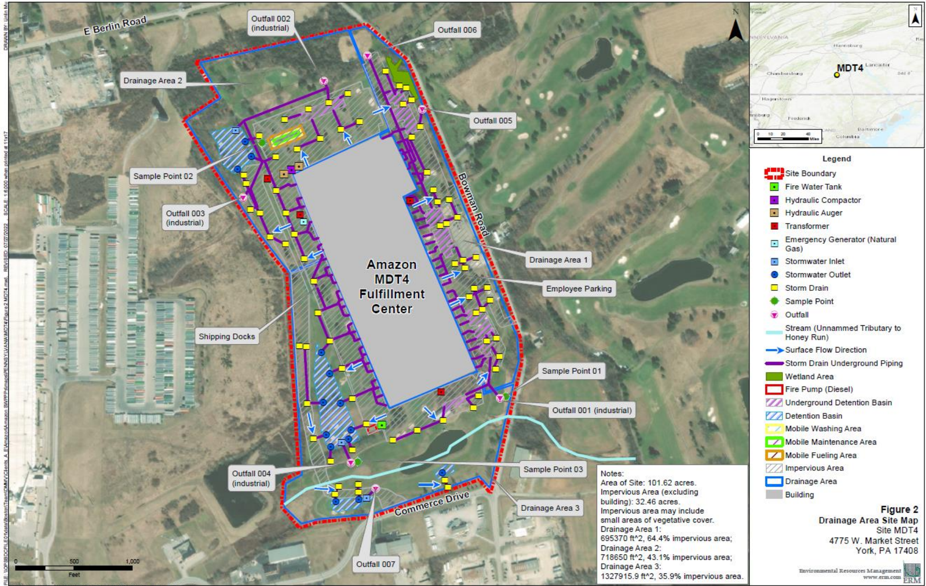
FIGURE 2. DRAINAGE AREA SITE MAP
