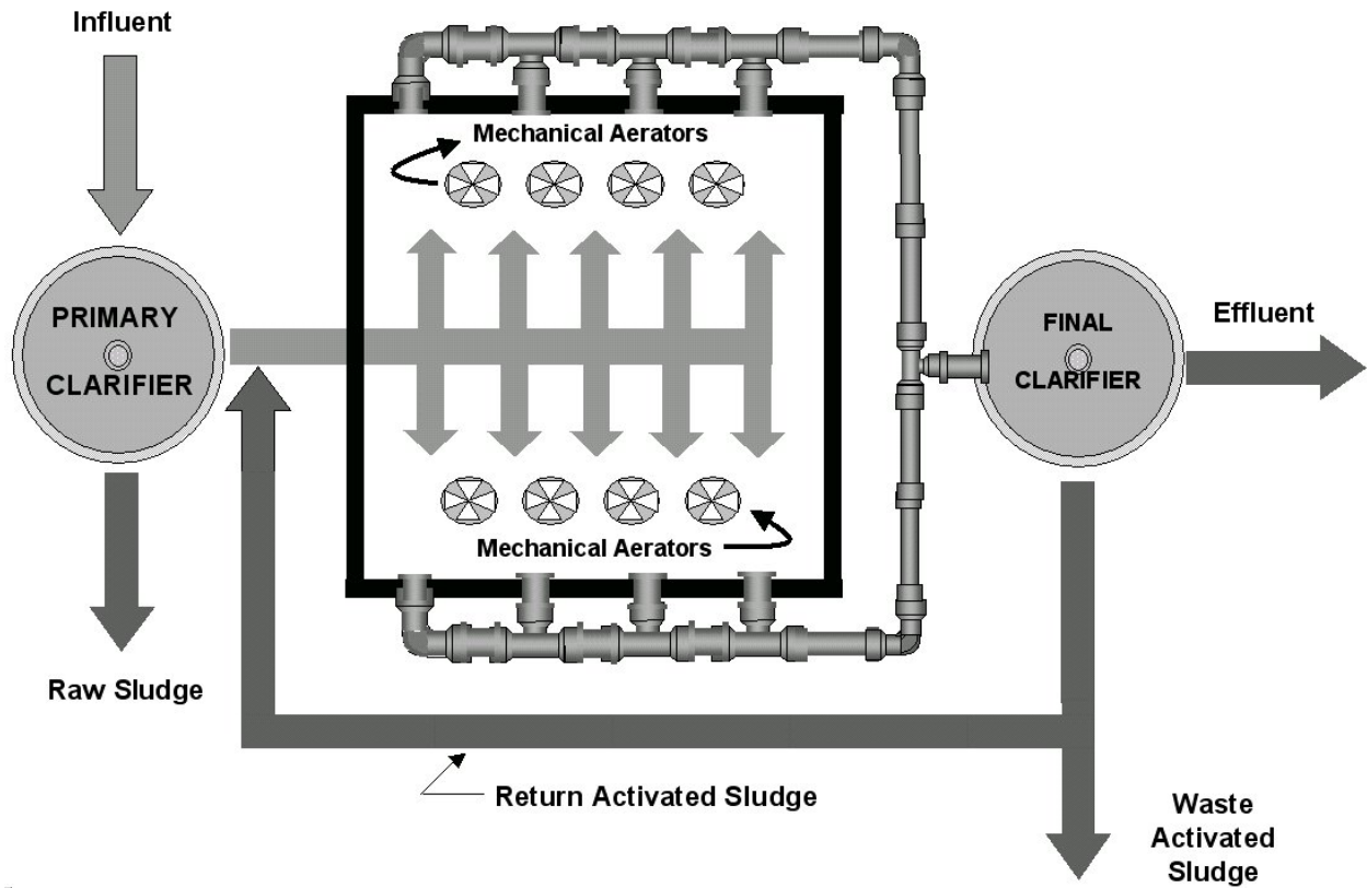
Schematic Drawing of a Completely-Mixed Aeration System
