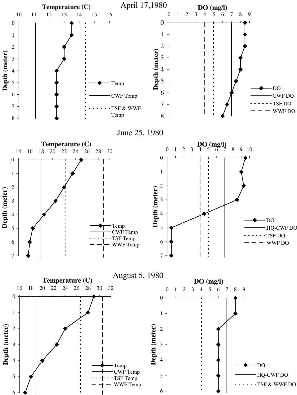
FIGURE 5. SPEEDWELL FORGE LAKE - WATER CHEMISTRY 1 Temperature and Dissolved Oxygen Profiles Ulanoski and Shertzer 1981
