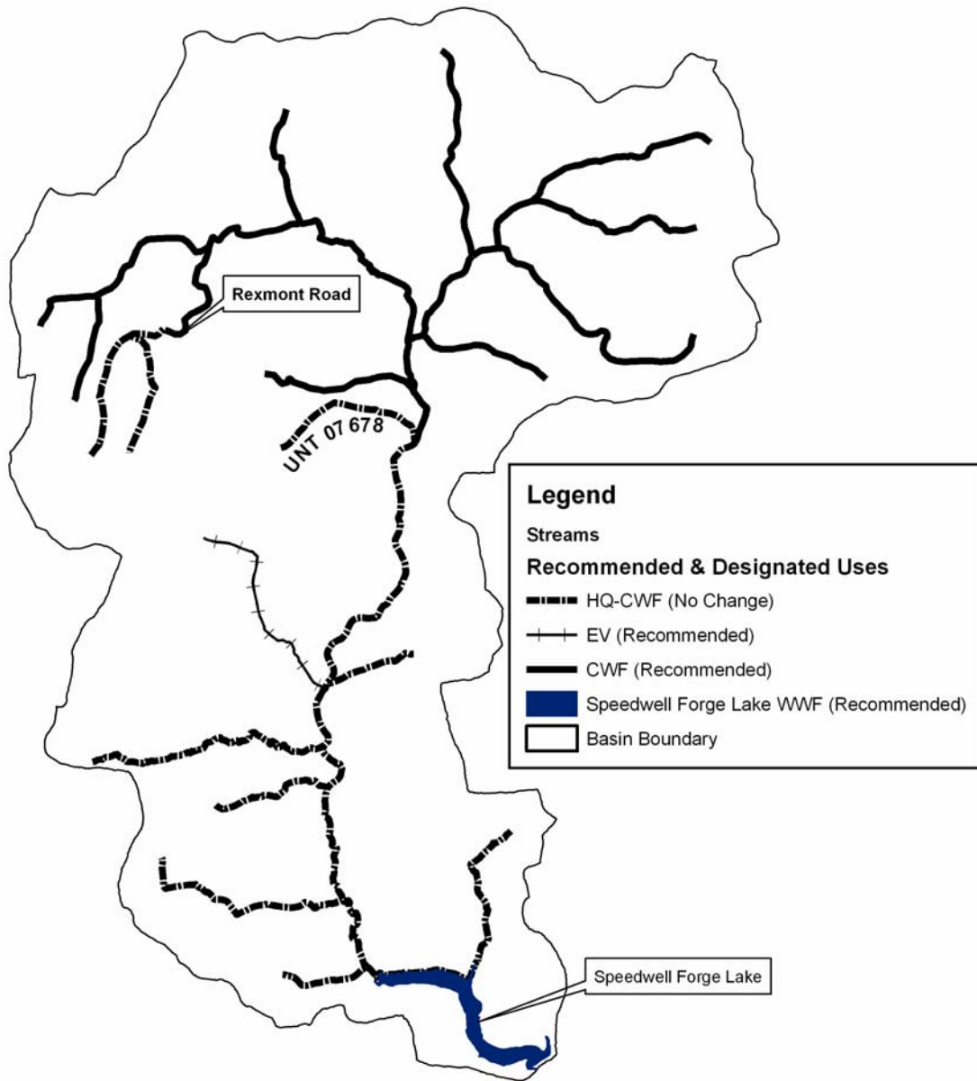
Figure 9. Hammer Creek Watershed
